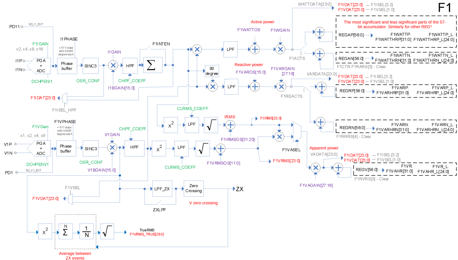
Figure 21 – Block diagram of F1
