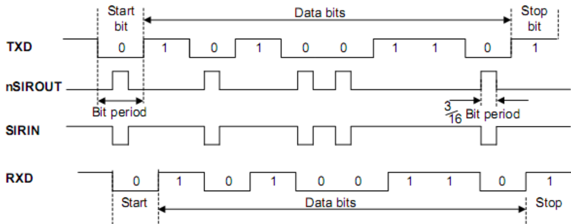
Figure 89 – IrDA data modulation
