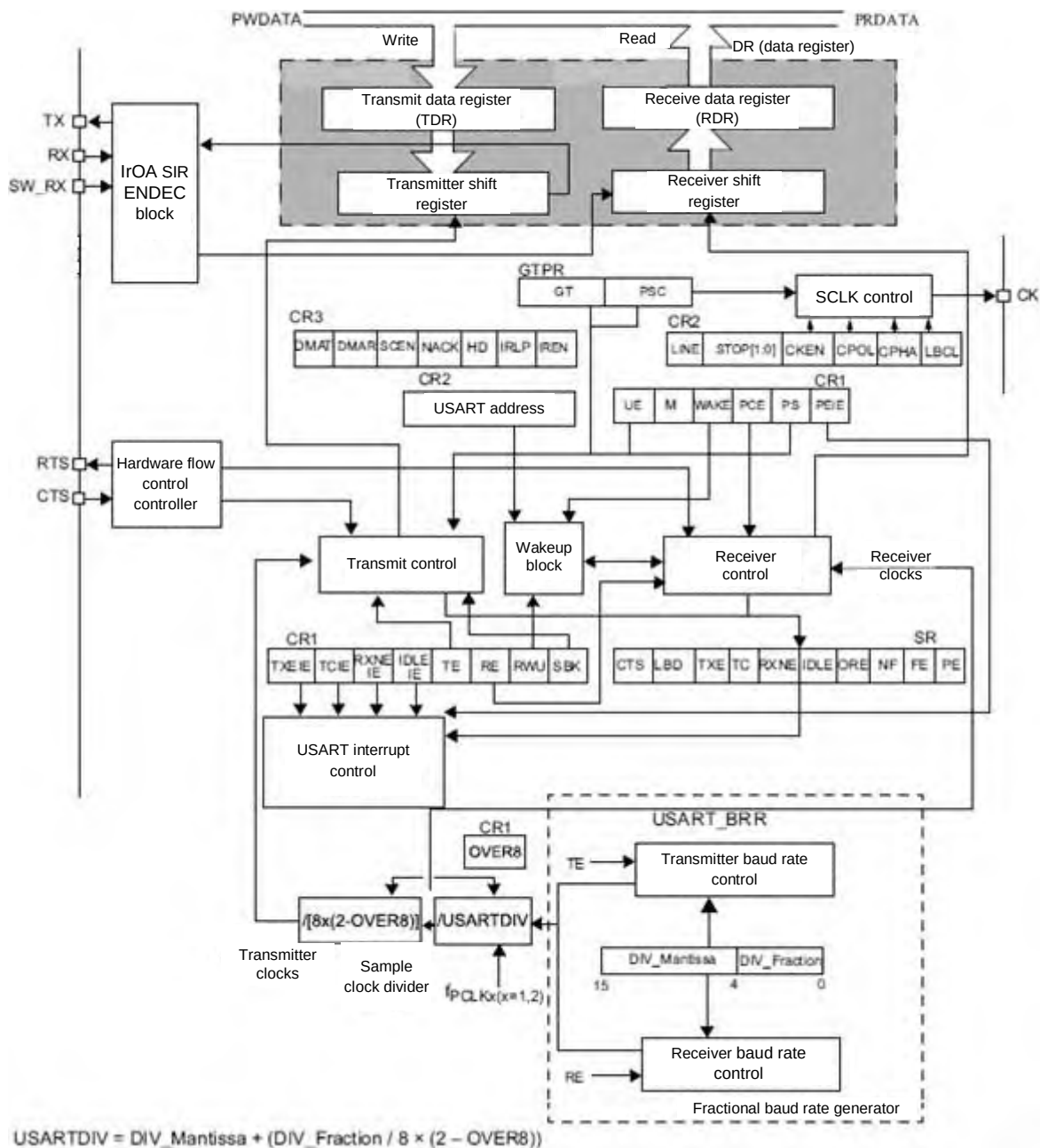
Figure 112 – USART block diagram
