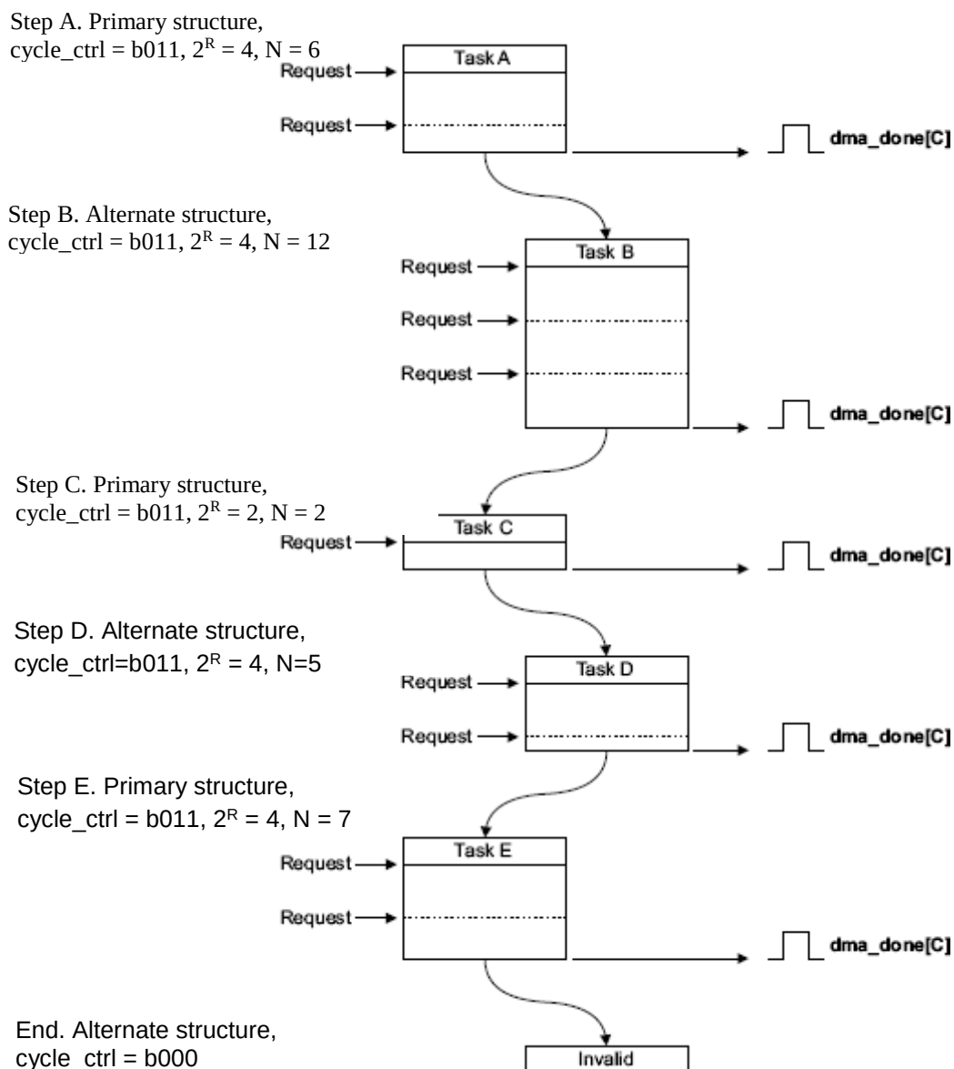
Figure 100 – Example of controller operation in ping-pong mode
