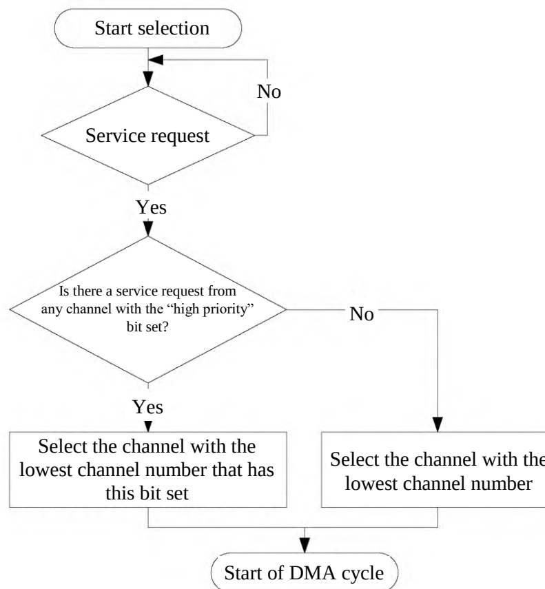
Figure 99 – Algorithm for selecting the next channel to be serviced
