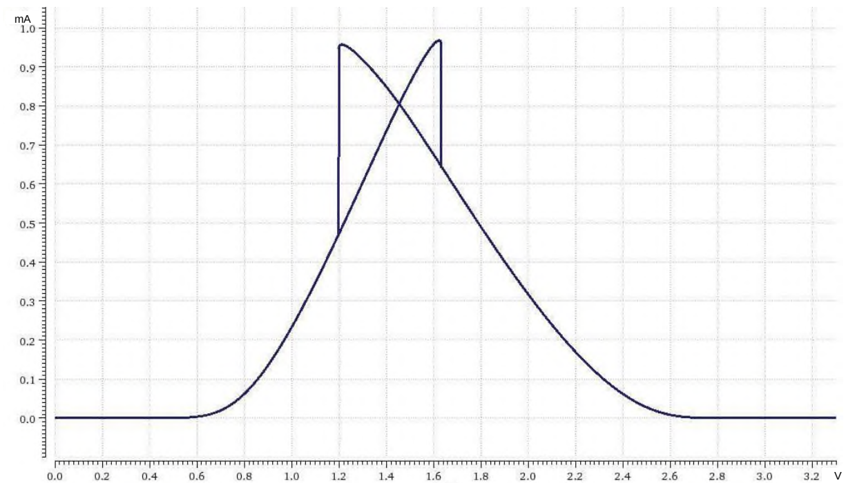
Figure 132 – Typical dependence of additional U_{CC} supply current on digital input voltage at U_{CC} = 3.3 V under nominal conditions
