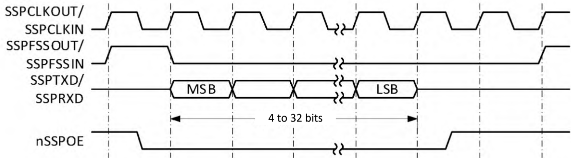
Figure 70 – SSI protocol synchronous transfer format (single transfer)
