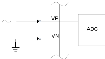
Figure 25 – Non-differential connection
