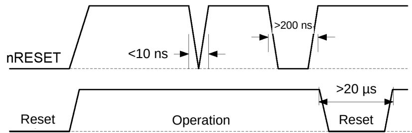
Figure 9 – Glitch filtering diagram for reset signal generation
