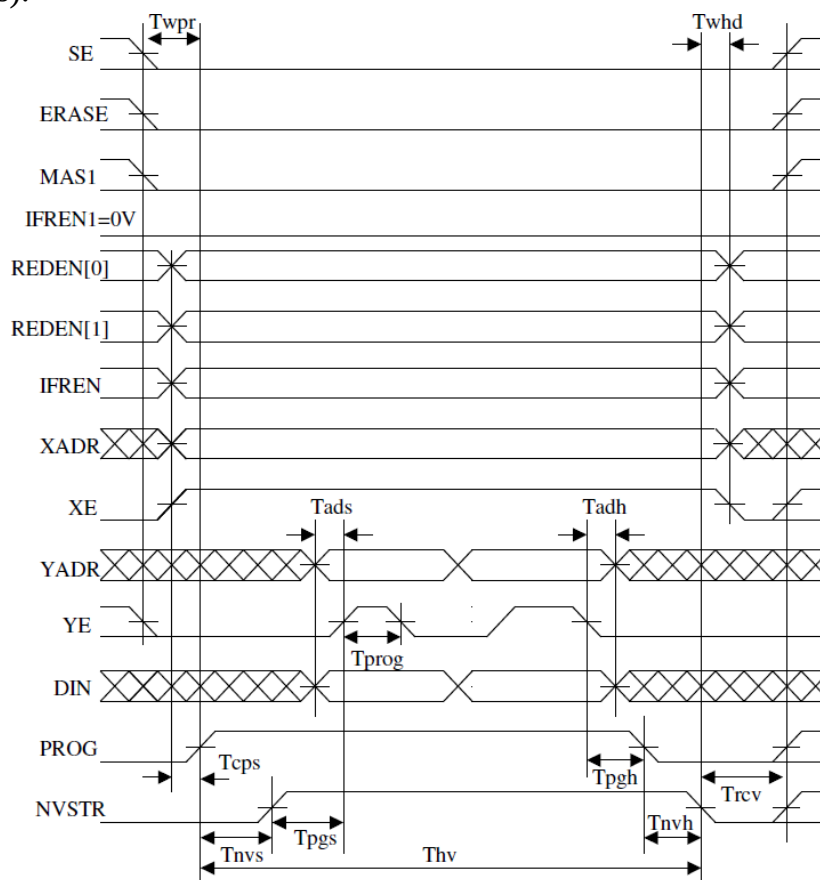
Figure 15 – Memory write timing diagram
