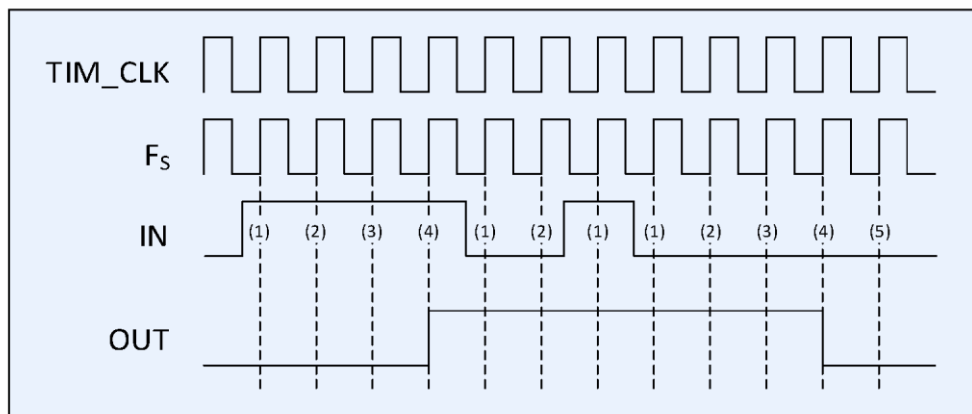
Figure 62 – Filter operation timing diagram, F_s = \text{TIM\_CLK} , N = 4
