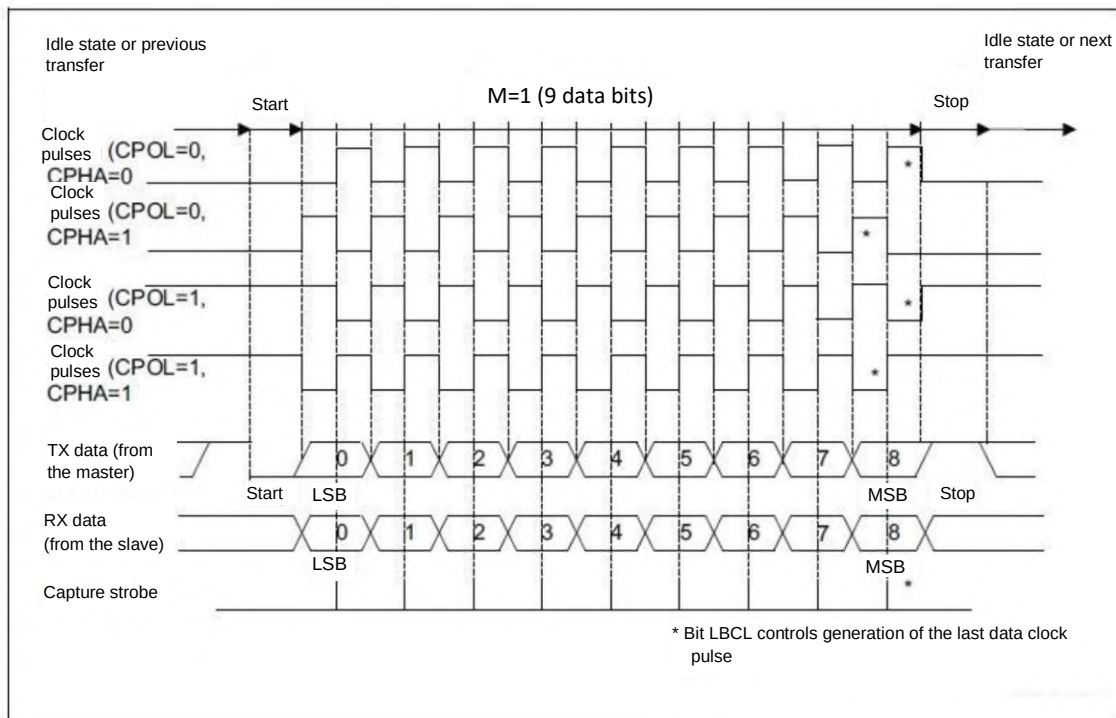
Figure 123 – USART data clocking diagram (M=1)
