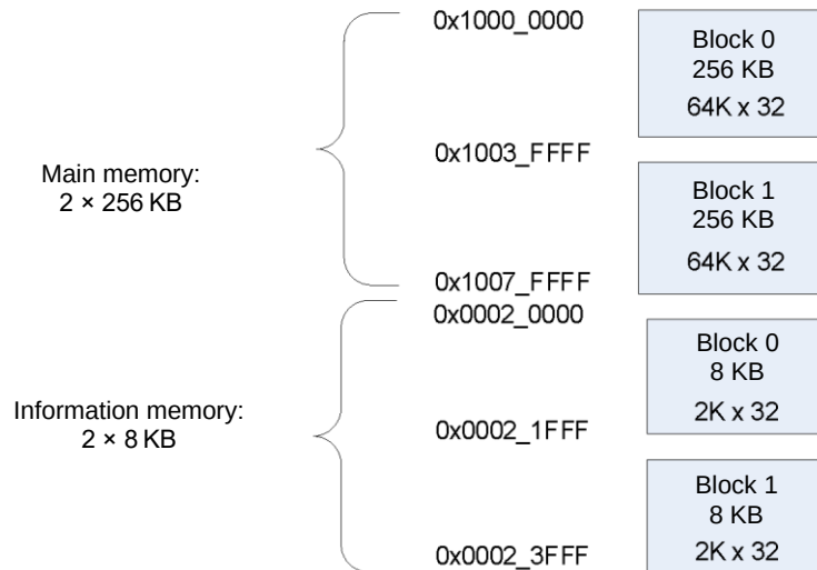
Figure 12 – Memory structure
