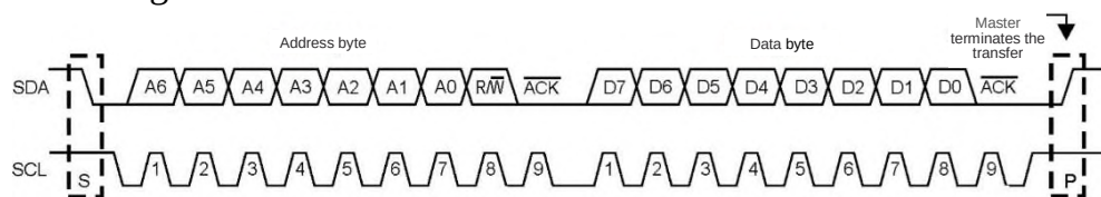
Figure 66 – I2C receive/transmit in 7-bit mode
