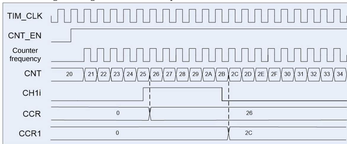
Figure 55 – Capture timing diagram for an event on channel 1 input
