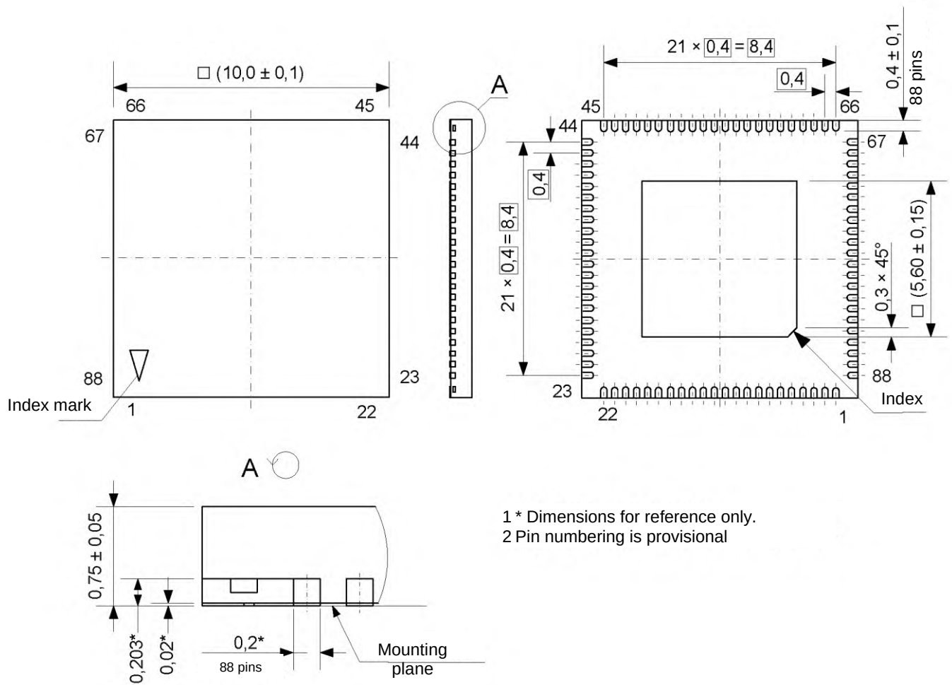
Figure 140 – IRL1206FI in QFN88 10×10×0.75 (0.4) package
