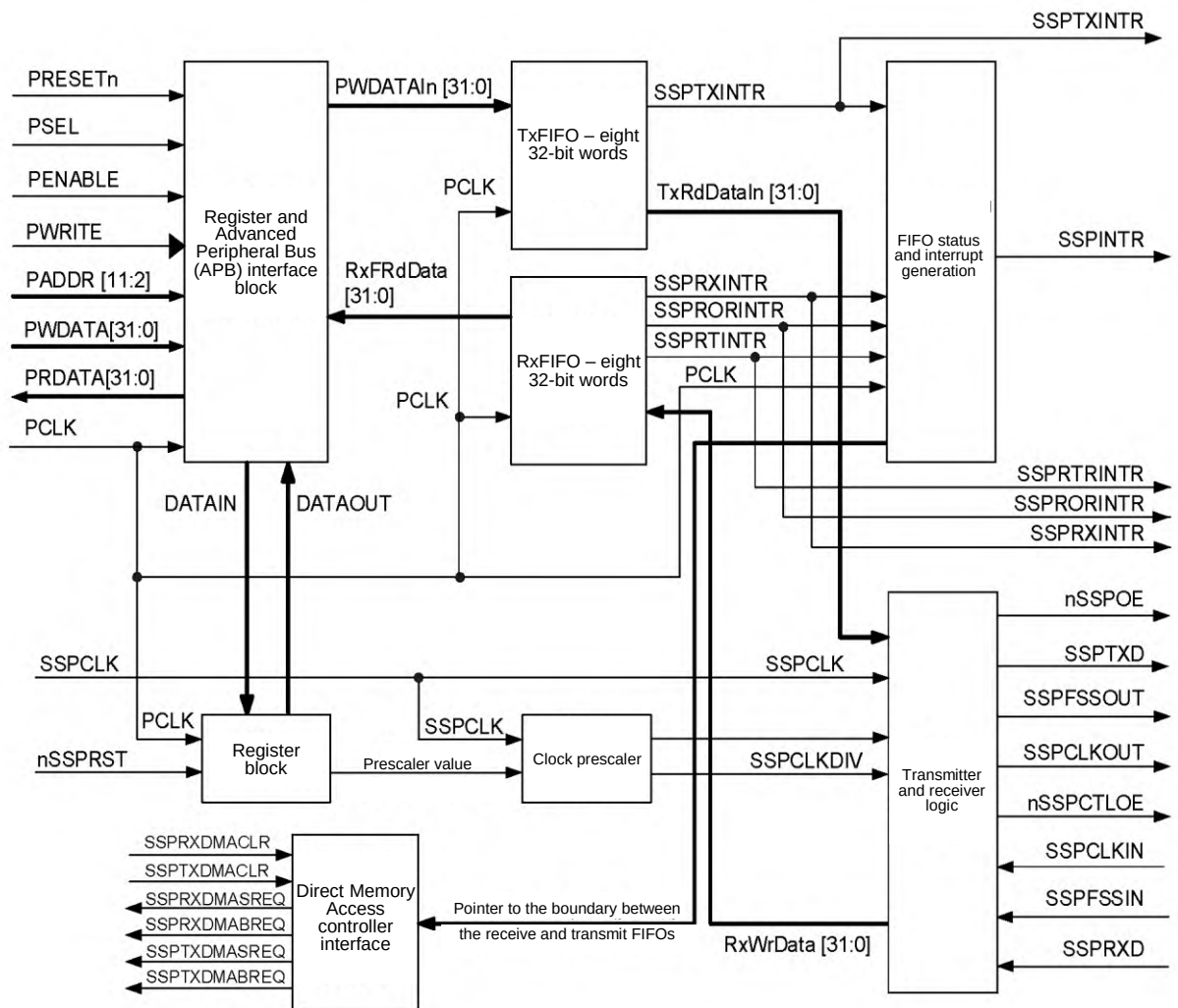
Figure 69 – SSP module block diagram
