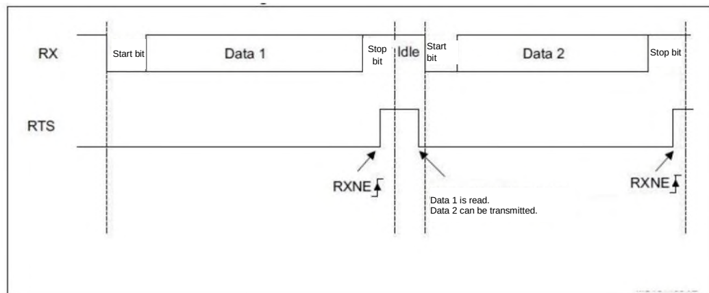
Figure 128 – RTS flow control
