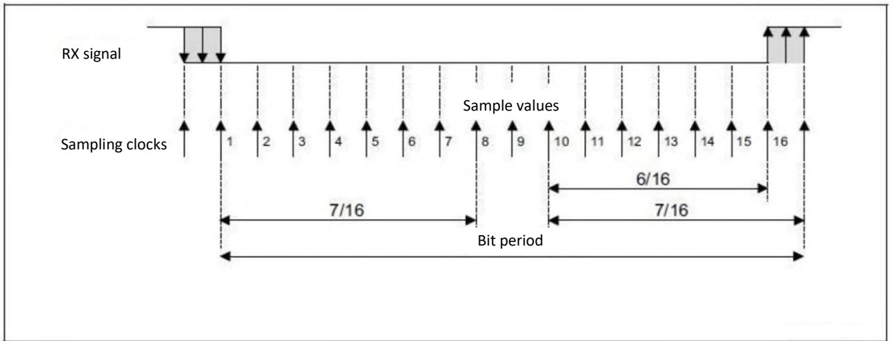
Figure 117 – Data sampling with oversampling by 16
