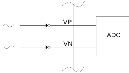
Figure 24 – Differential connection
