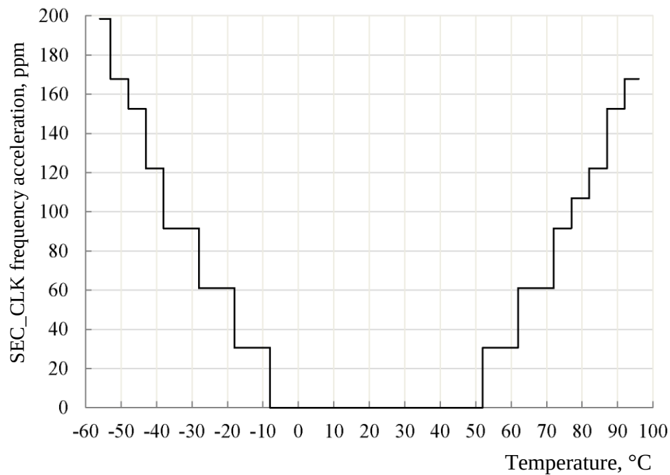
Figure 35 – Typical dependence of SEC_CLK frequency correction (acceleration) on temperature at BKP_RTC_PRL = 32767
