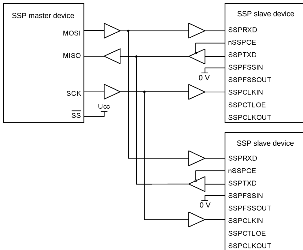
Figure 83 – SPI master device connected to two SSP slave modules
