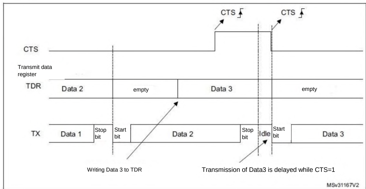
Figure 129 – CTS flow control
