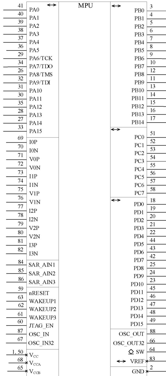
Figure 2 – Conventional graphical representation of IRL1206FI
