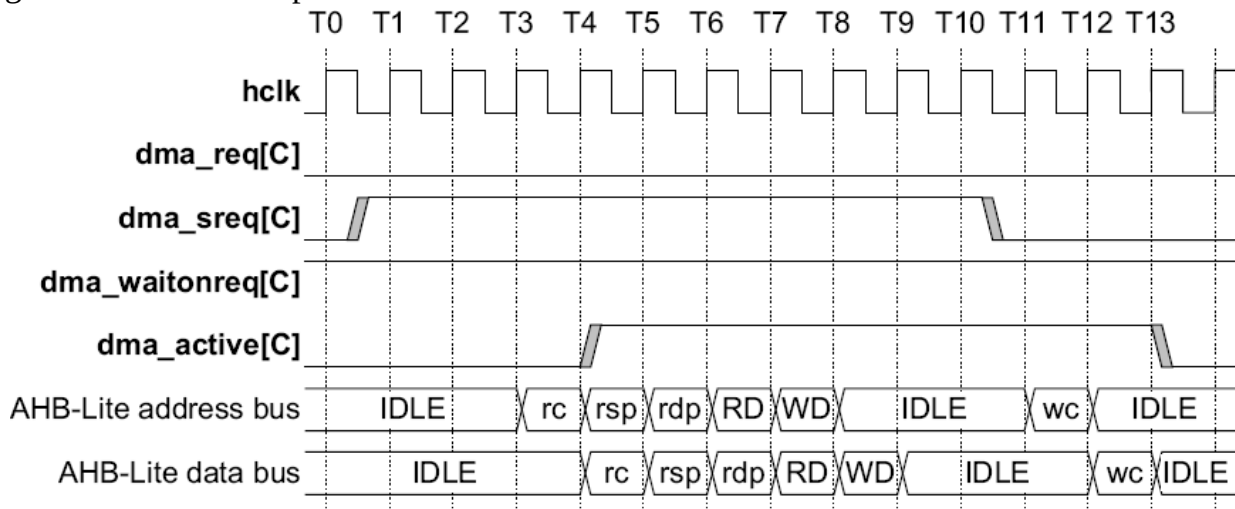
Figure 98 – DMA operation when dma_waitonreq is used together with dma_sreq
