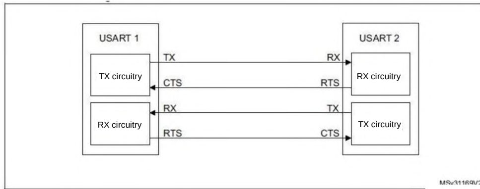
Figure 127 – Hardware data flow control between two USART devices
