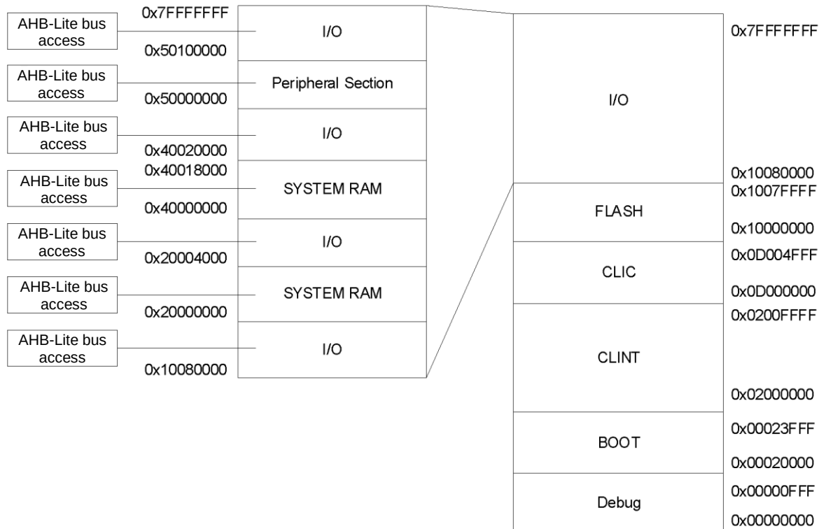
Figure 11 – Address space structure of the integrated circuit
