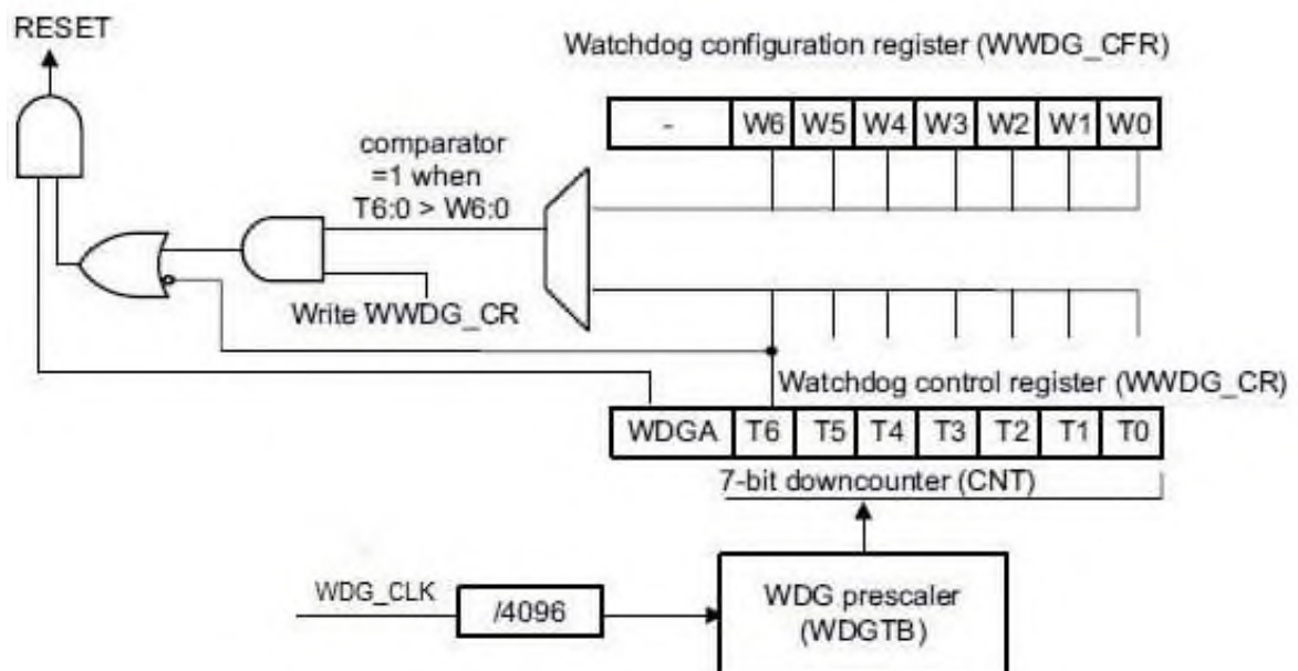
Figure 109 – Block diagram of the window watchdog timer
