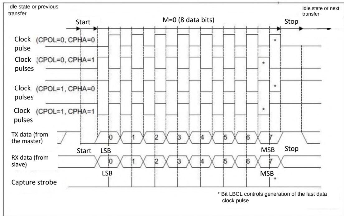
Figure 122 – USART data clocking diagram (M=0)
