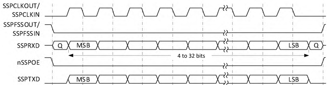
Figure 74 – SPI protocol synchronous transfer format, SPO=0, SPH=1
