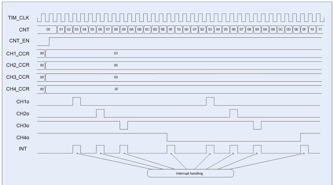
Figure 66 – Example timing diagrams in PWM mode
