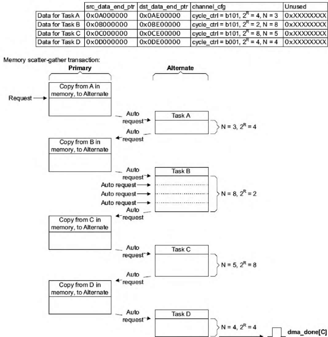
Figure 101 – Example of DMA operation in “Execution with configuration change” mode
