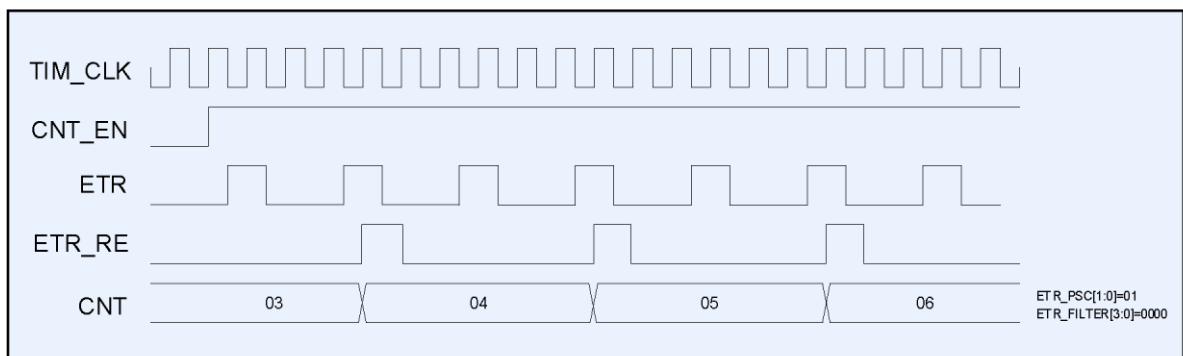
Figure 53 – Clocking diagram from the ETR input, EVNT\_SEL[3:0] = 1000
