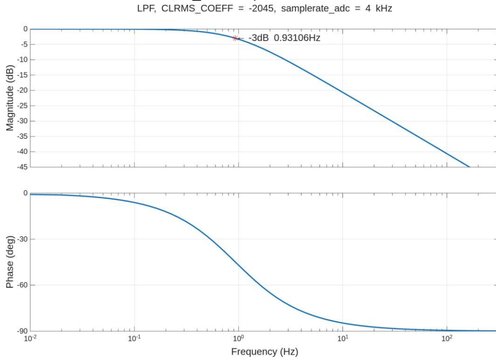
Figure 19 – Amplitude and phase frequency responses of the LPF filter with default settings at 4 kHz
