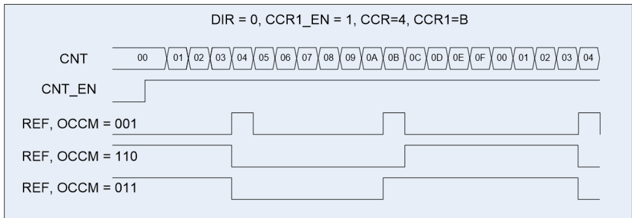
Figure 58 – PWM operation timing diagram, CCR1_EN = 1
