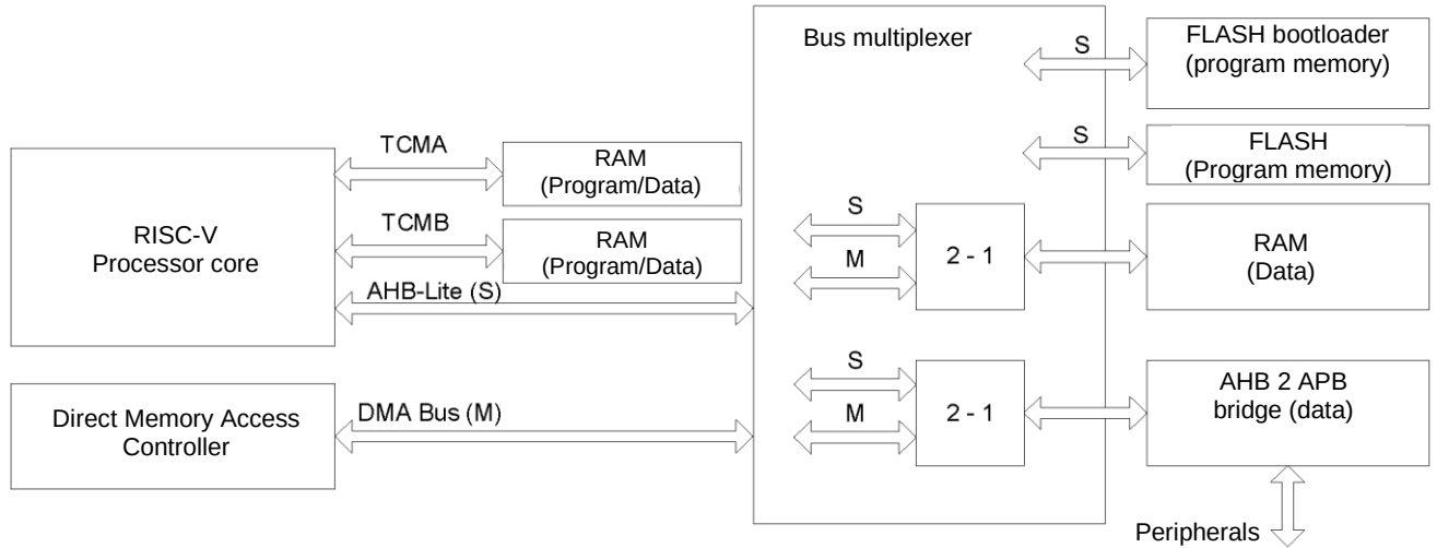
Figure 10 – Memory organization block diagram
