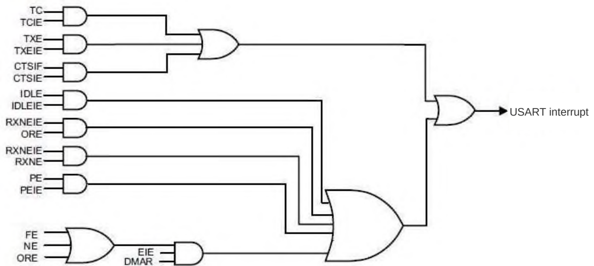
Figure 130 – Diagram of USART events to the interrupt
