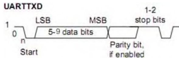
Figure 88 – Data frame
