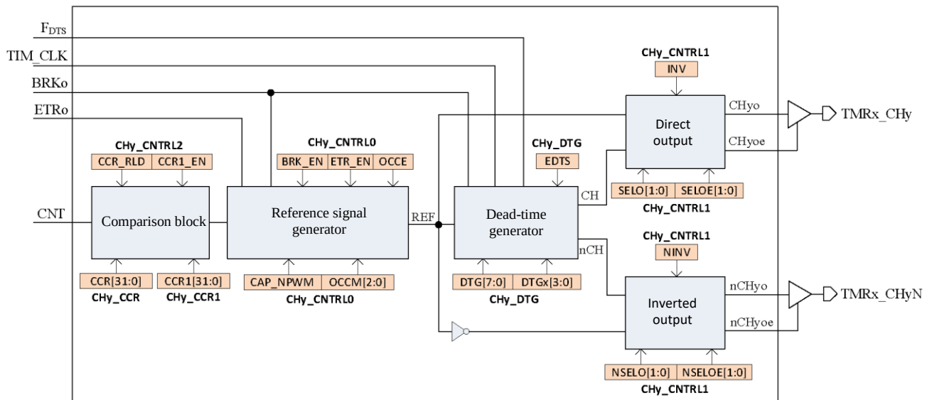
Figure 56 – Block diagram of the PWM generation block
