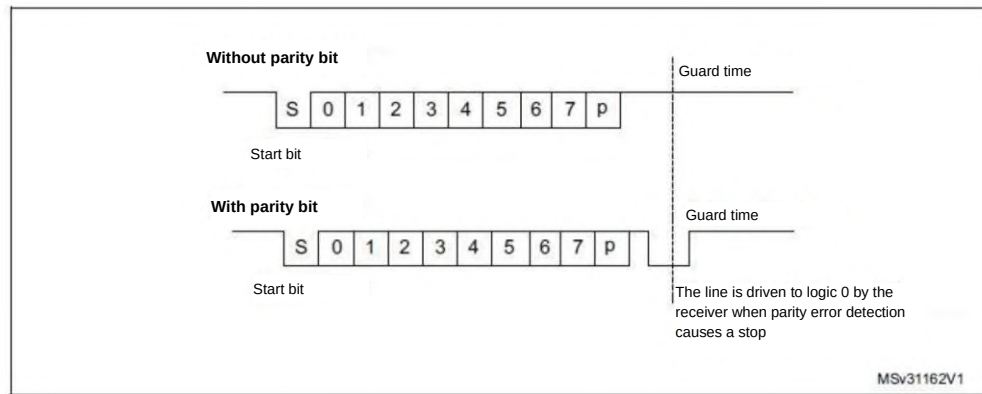
Figure 125 – ISO 7816-3 asynchronous protocol
