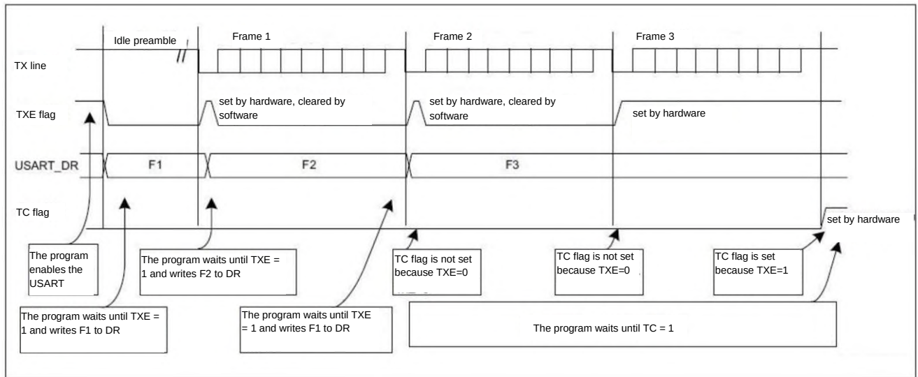
Figure 115 – TC/TXE status during transmission
