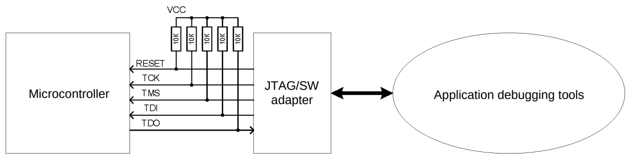
Figure 107 – Debug mode operation diagram
