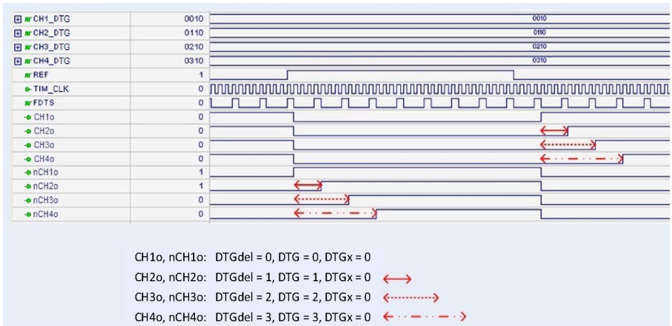
Figure 61 – DTG block operation timing diagram
