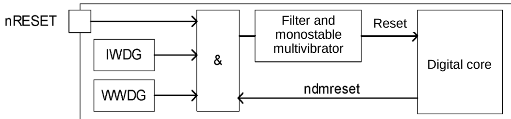
Figure 8 – Reset generation block diagram
