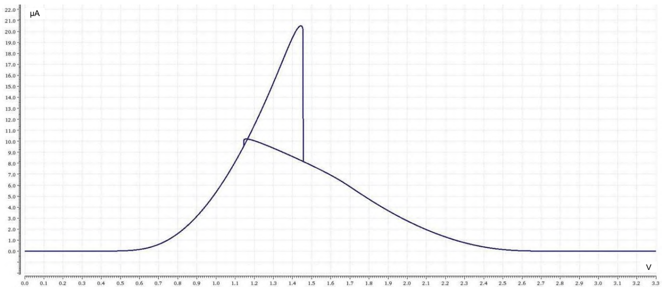
Figure 133 – Typical dependence of additional U_{CCB} supply current on WAKEUP1-WAKEUP3 input voltage at U_{CCB} = 3.3 V under nominal conditions
