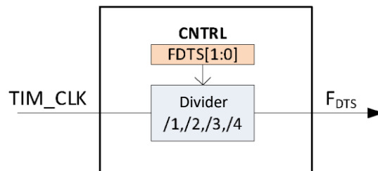
Figure 43 – F DTS clock generation scheme
