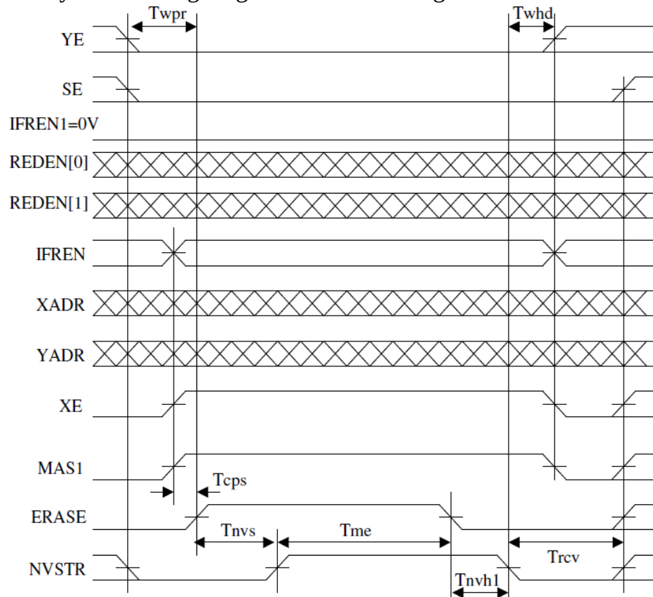
Figure 13 – Memory erase timing diagram
