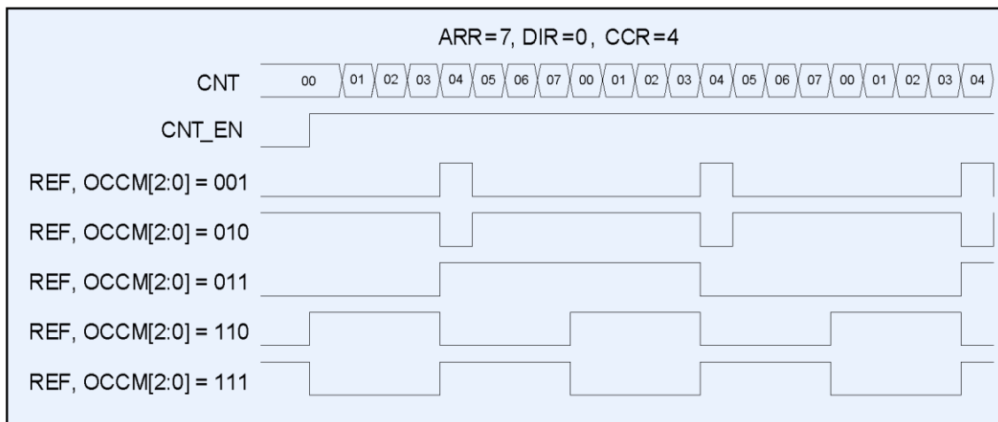
Figure 57– PWM operation timing diagram, CCR1_EN = 0
