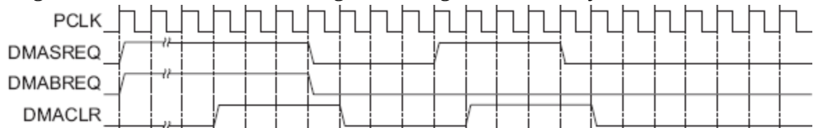
Figure 84 – DMA mode transfer timing diagrams
