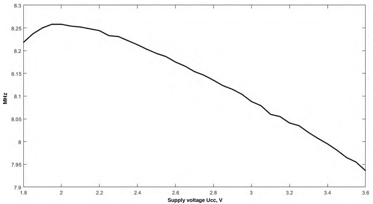
Figure 136 – Dependence of HSI RC oscillator frequency of IRL1206FI (CHIP_ID = 217) on supply voltage U_{CC} under nominal conditions
