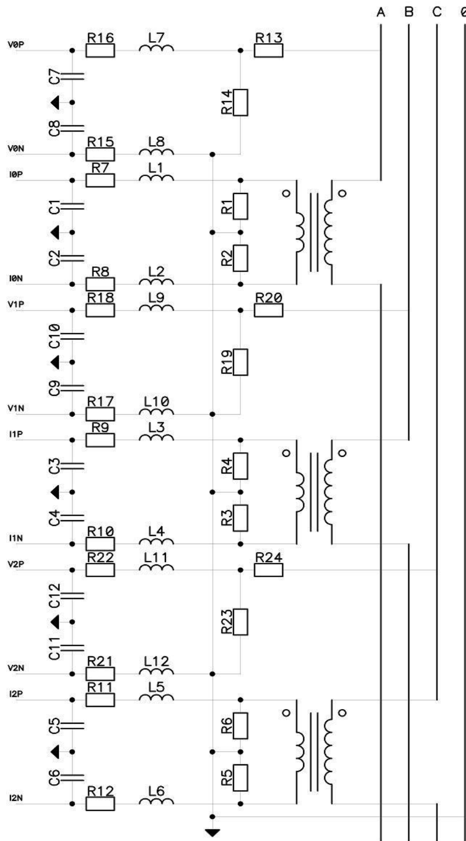
Figure 30 – Typical connection diagram for three-phase electric power metering
