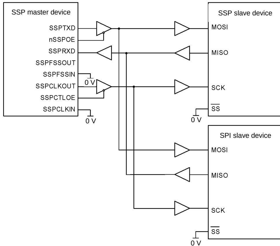
Figure 82 – SSP master device connected to two slaves supporting SPI
