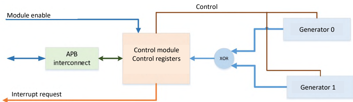
Figure 111 – Block diagram of the random number generator block
