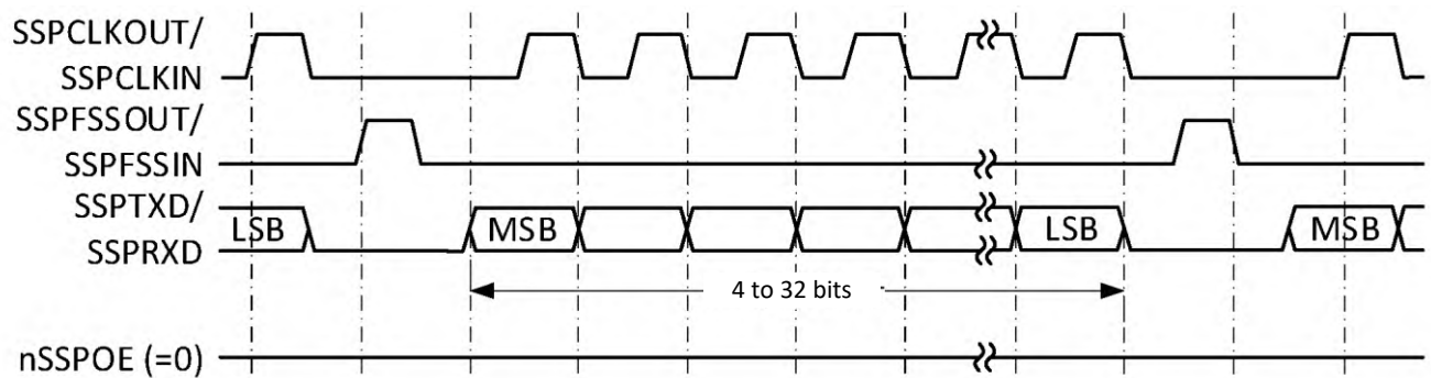
Figure 73 – SPI protocol synchronous transfer format, SPO = 0, SPH = 0 (continuous transfer)
