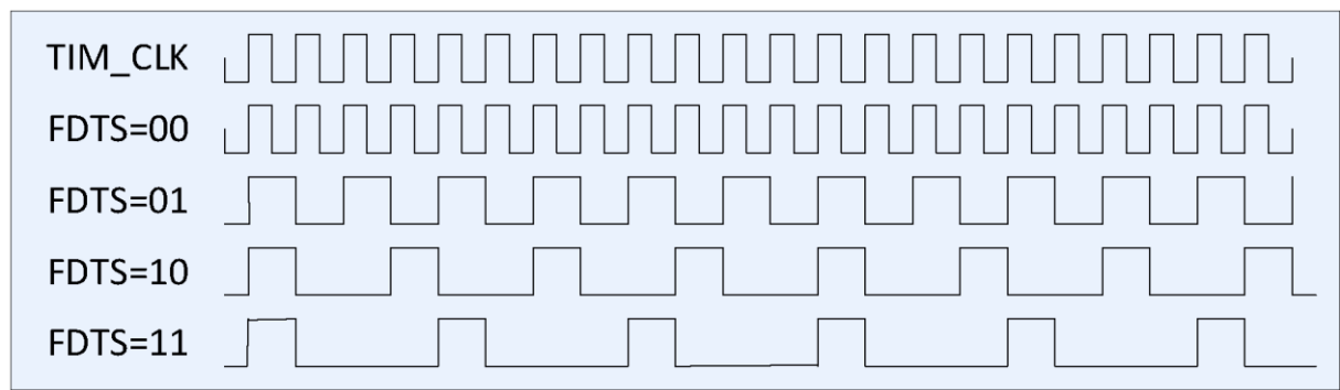
Figure 44 – FDTs clock frequency as a function of the FDTs[1:0] value in the CNTRL register
