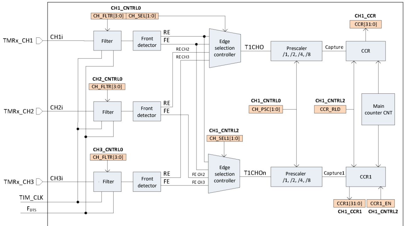
Figure 54 – Block diagram of the capture block (example for channel 1)
