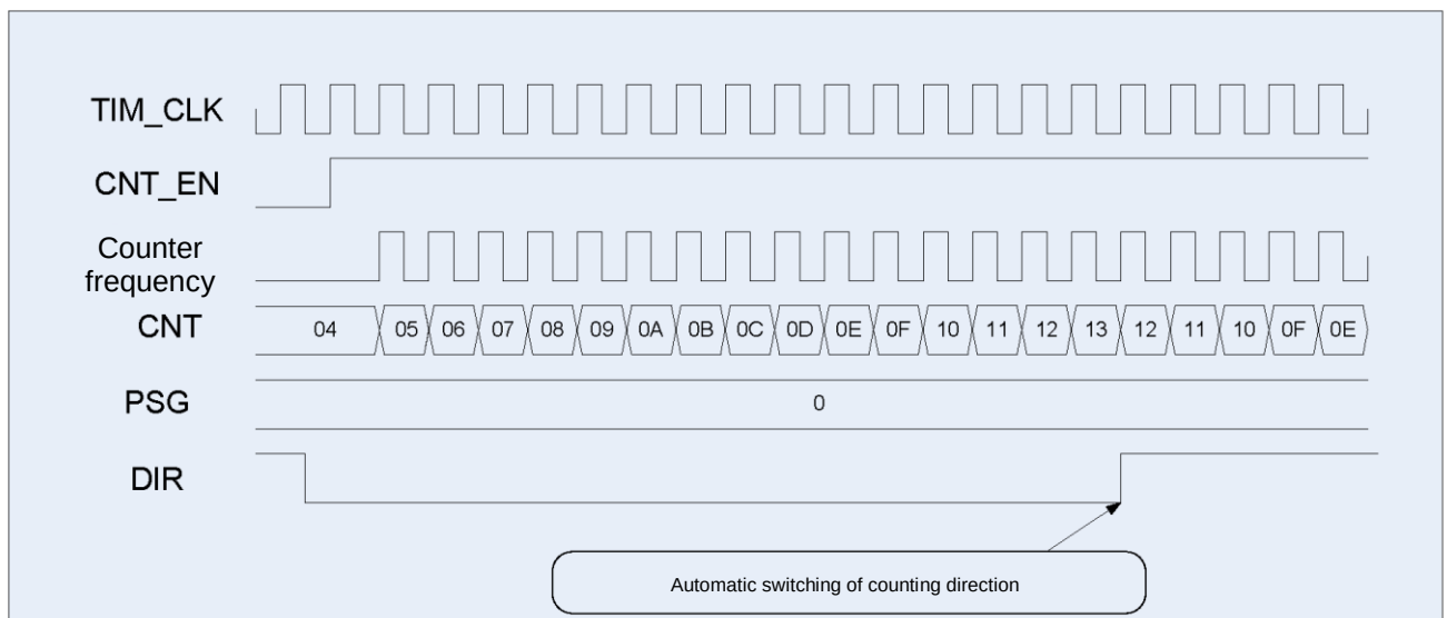
Figure 41 – Timer operation diagrams, bidirectional counting, starting with up-counting
