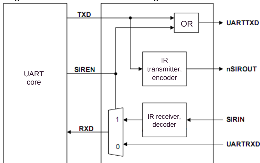
Figure 86 – IrDA codec block diagram
