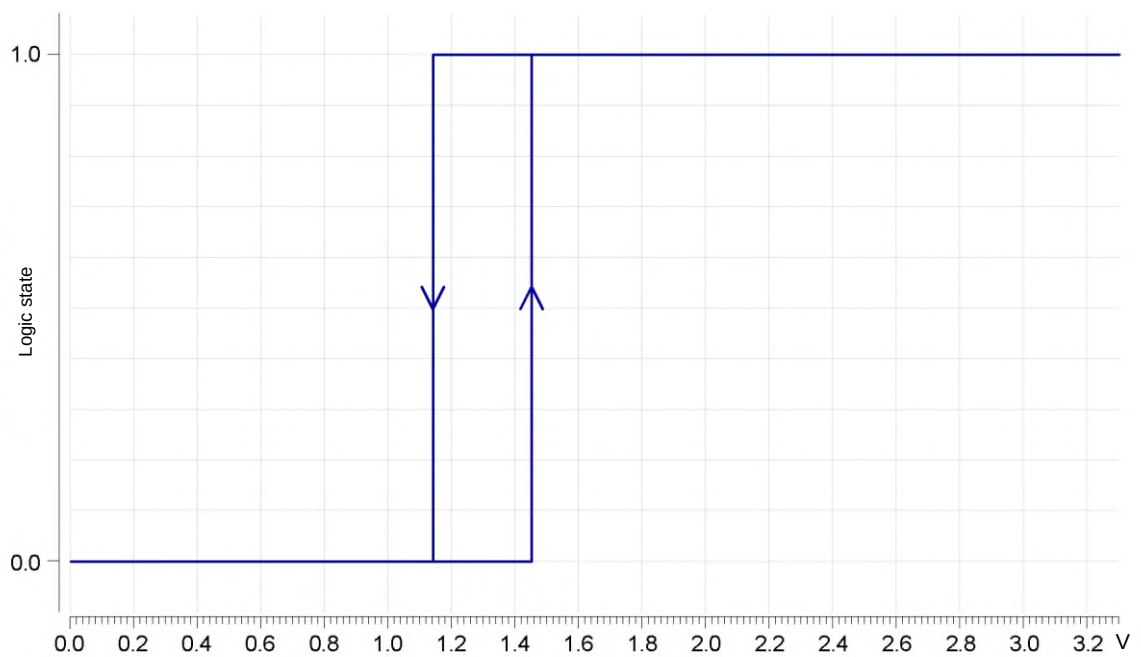
Figure 135 – Typical dependence of logic state on WAKEUP1-WAKEUP3 input voltage at U_{CCB} = 3.3 V under nominal conditions
