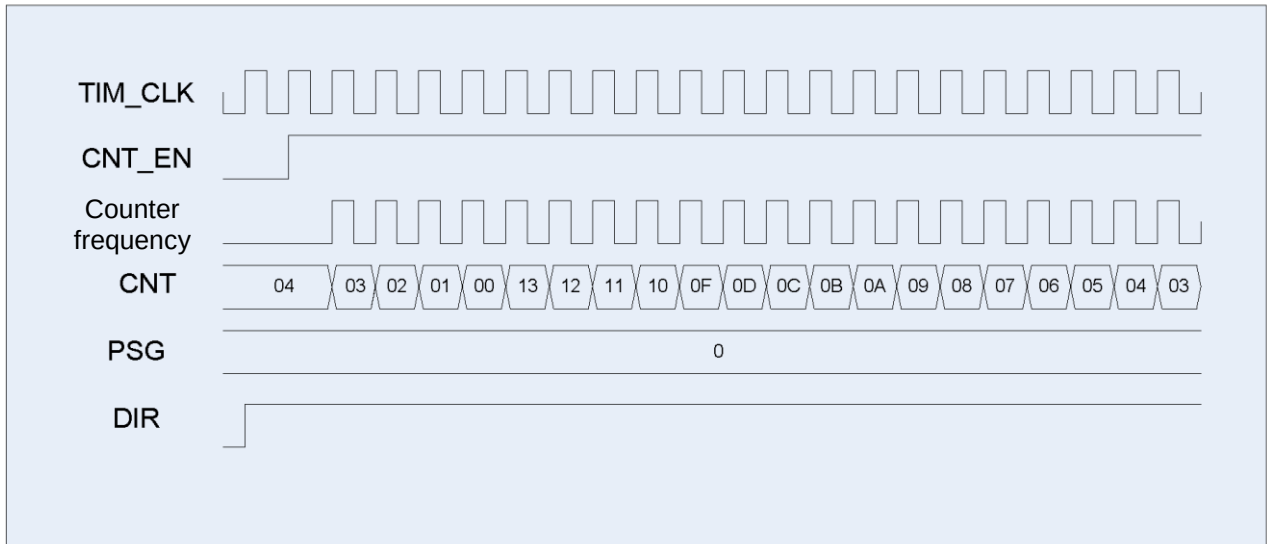
Figure 40 – Timer operation diagrams, down-counting from 0x13 to 0, start value 0x04
