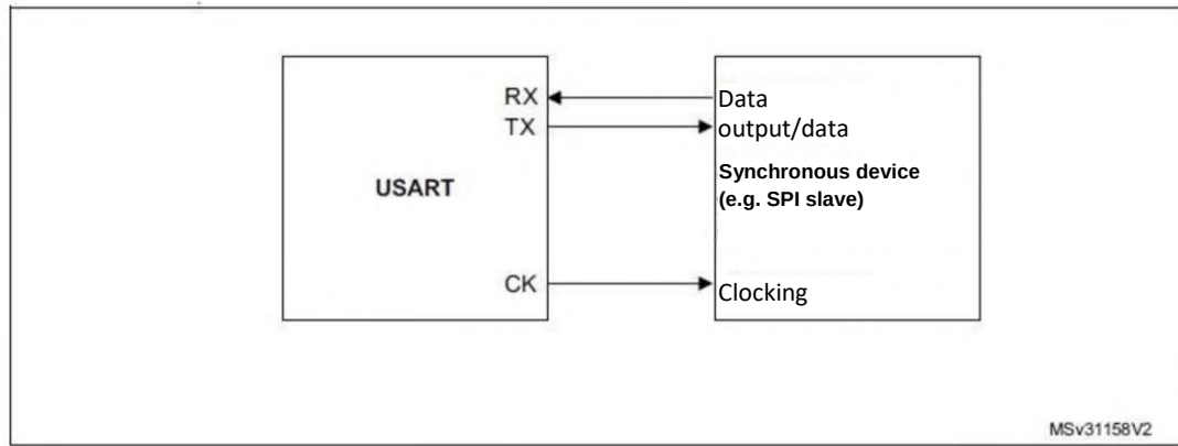
Figure 121 – Example of USART synchronous transfer
