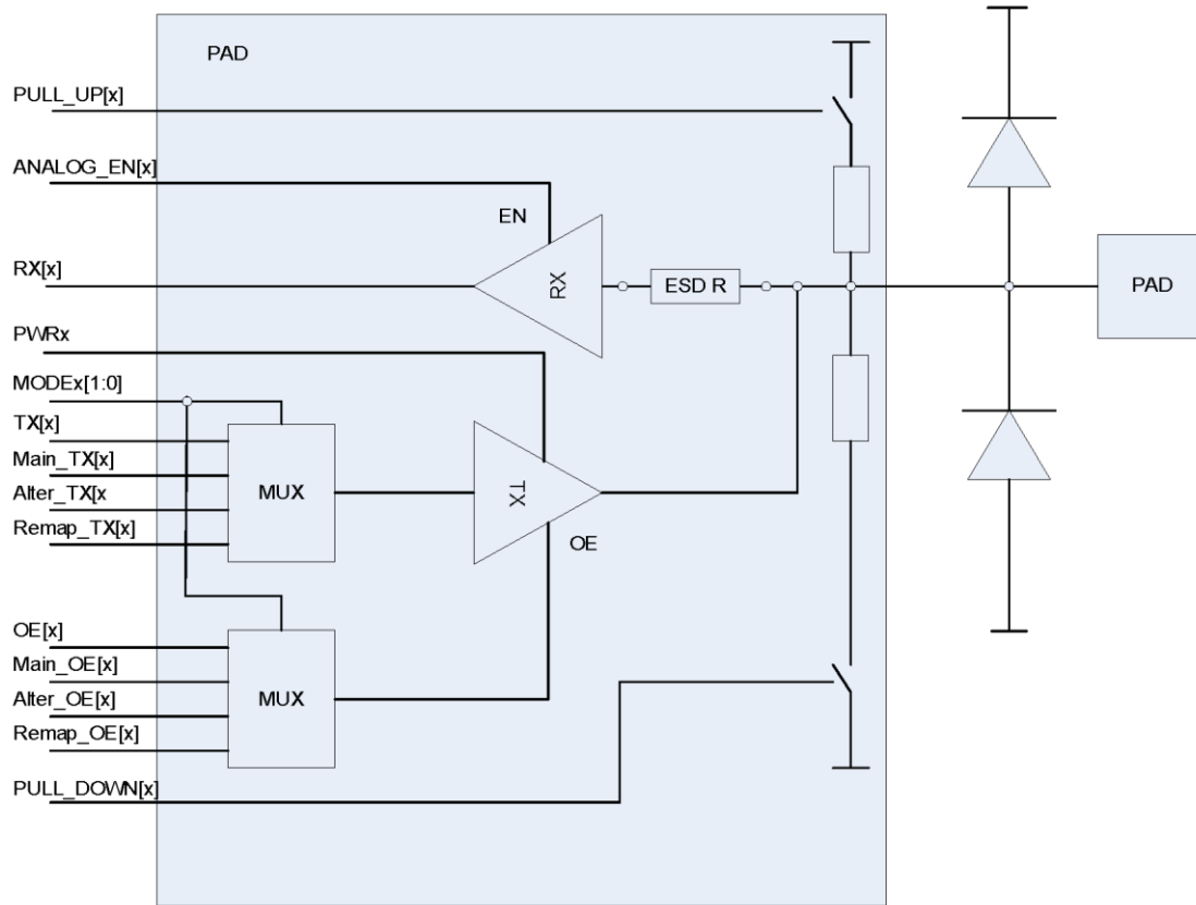
Figure 37 – Block diagram of an input/output port bit
