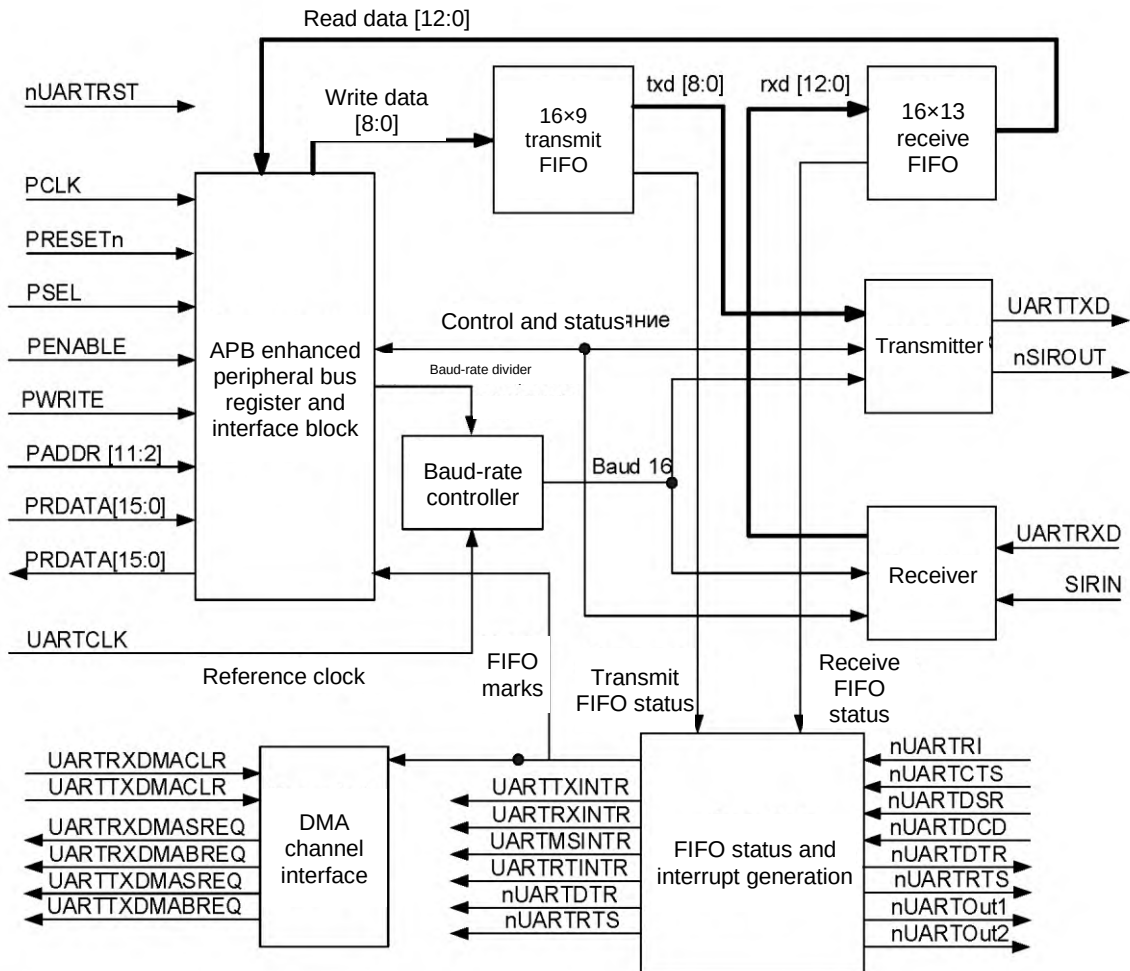
Figure 85 – Block diagram of the universal asynchronous receiver-transmitter (UART)
