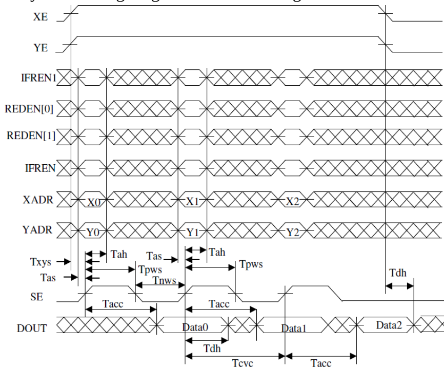
Figure 16 – Memory read timing diagram
