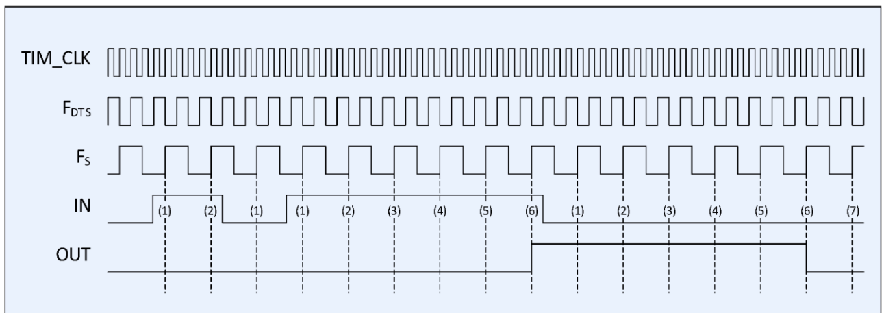
Figure 63 – Filter operation timing diagram, F_s = F_{DTS}/2 , N = 6
