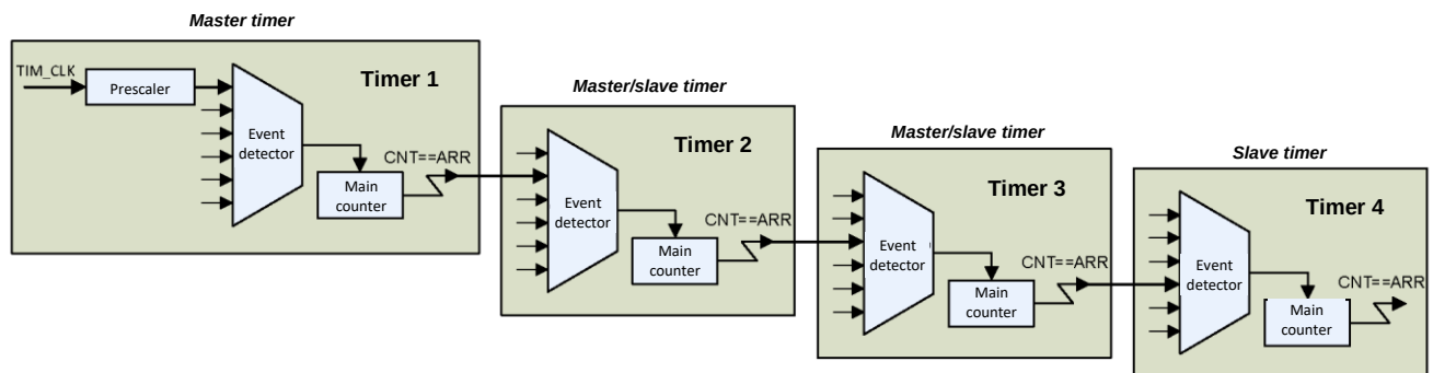
Figure 48 – Example of cascaded connection of timers
