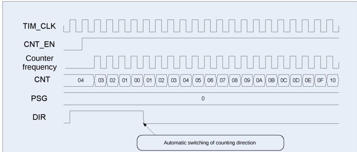
Figure 42 – Timer operation diagrams, bidirectional counting, starting with down-counting
