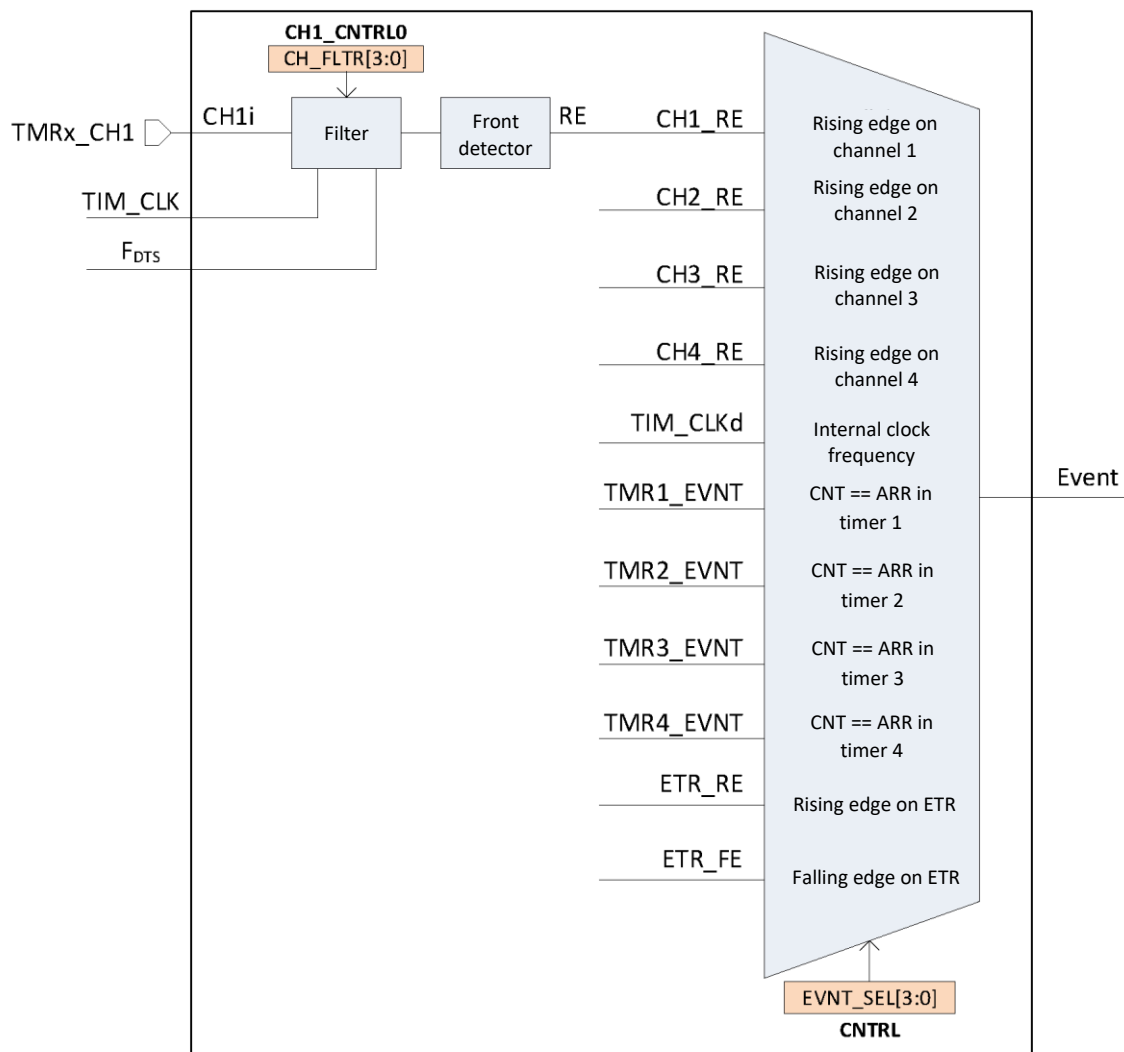
Figure 50 – Clocking scheme from the first channel input
