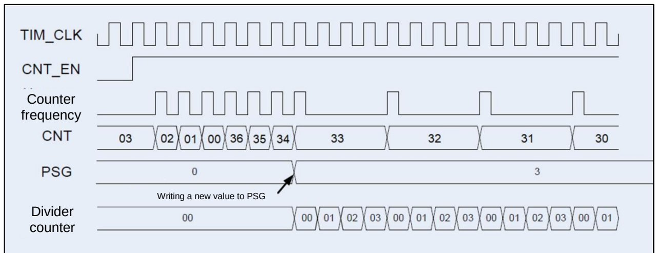
Figure 47 – Counter operation diagram: down-counting (CNT_MODE[1:0] = 00, EVNT_SEL[3:0] = 0000, DIR = 1)
