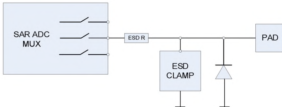
Figure 65 – SAR_AINx pin block diagram
