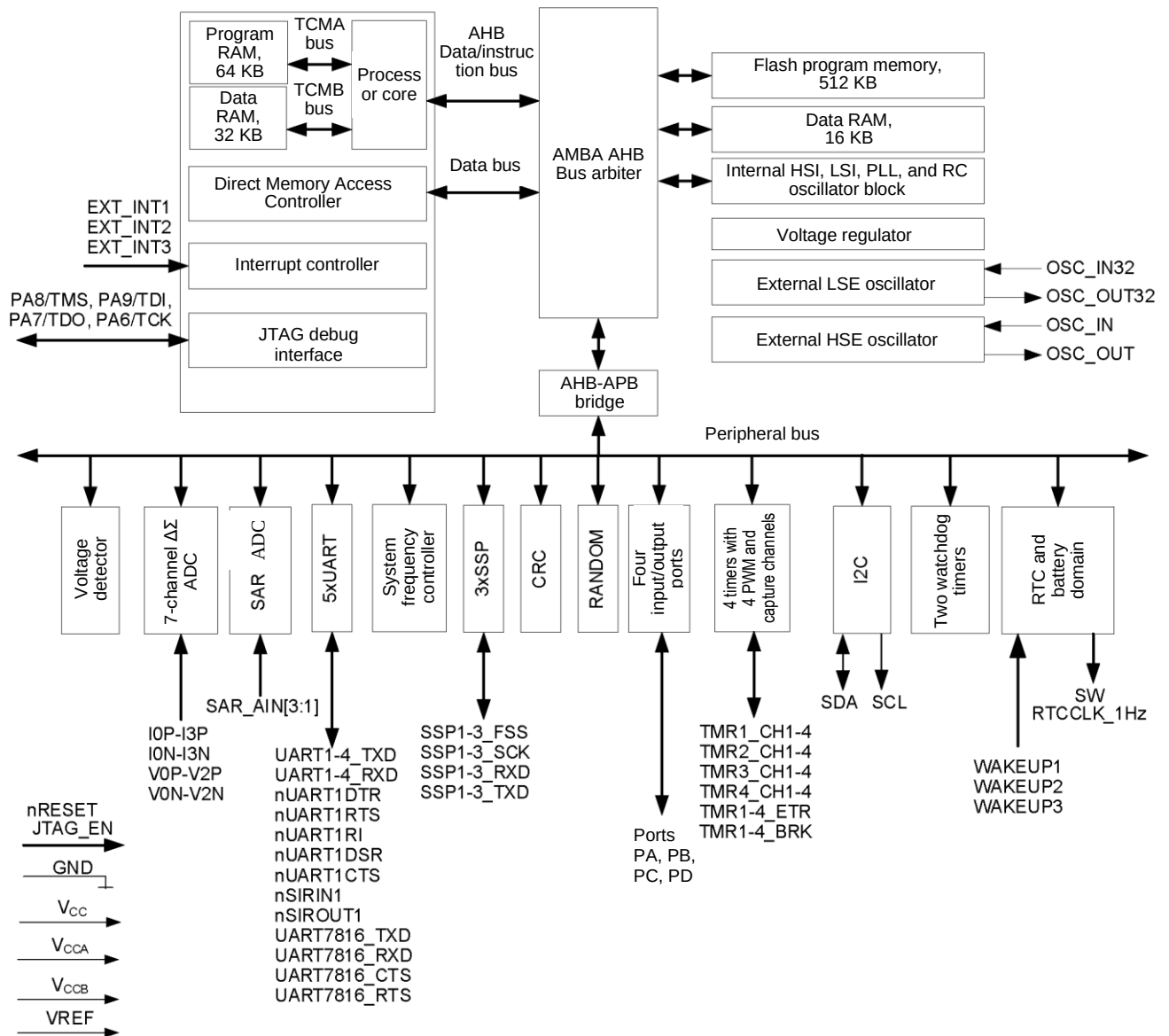
Figure 1 – Block diagram of IRL1206FI
