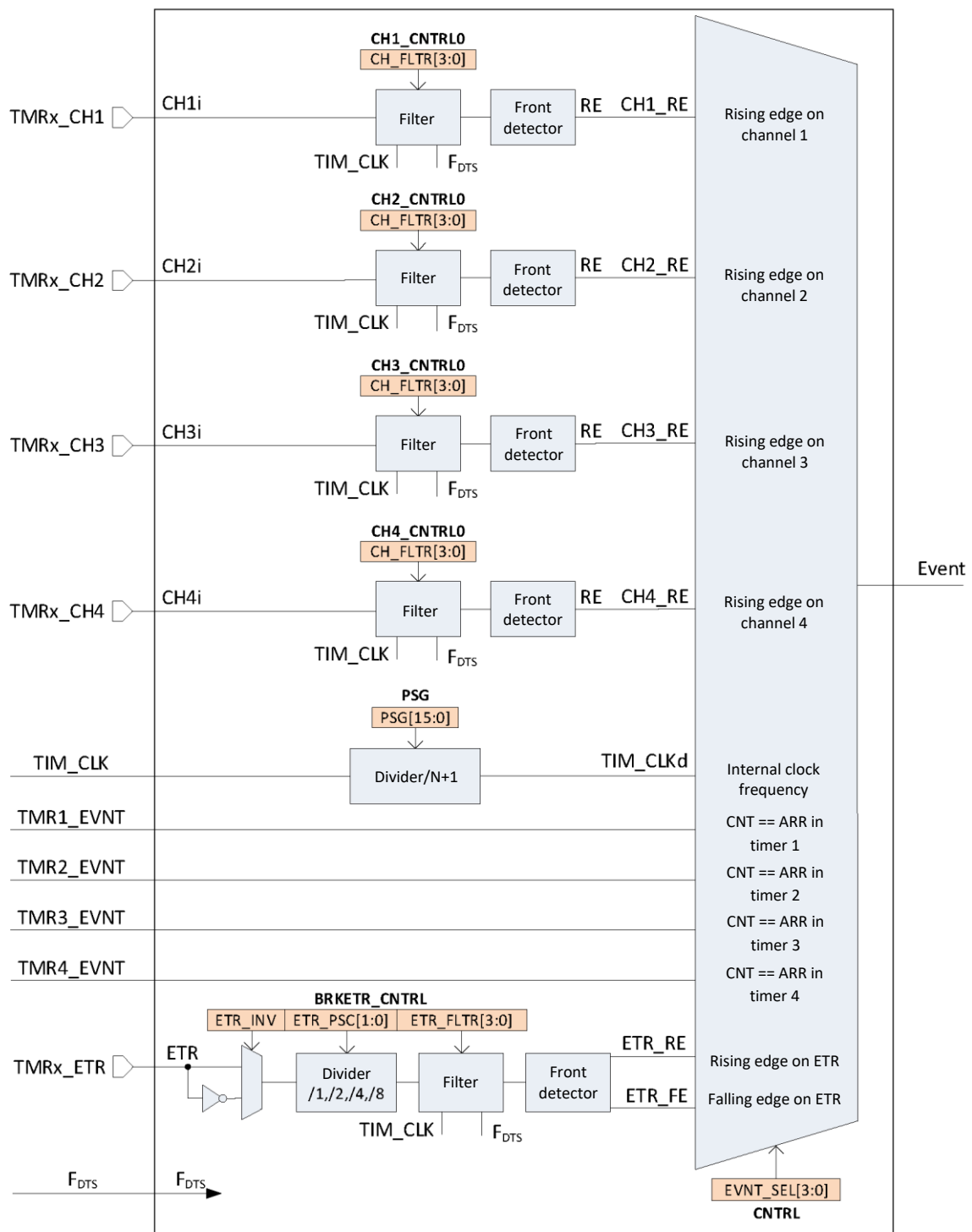
Figure 45 – Block diagram of event generation for counting
