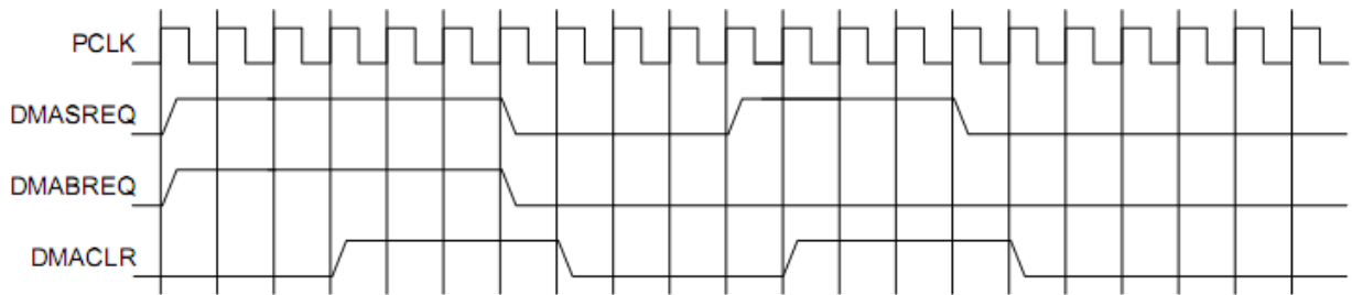
Figure 91 – Timing diagrams for single-word and block DMA requests
