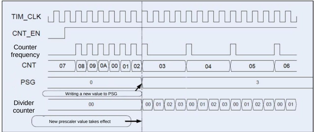
Figure 46 – Counter operation diagram: up-counting (CNT_MODE[1:0] = 00, EVNT_SEL[3:0] = 0000, DIR = 0)
