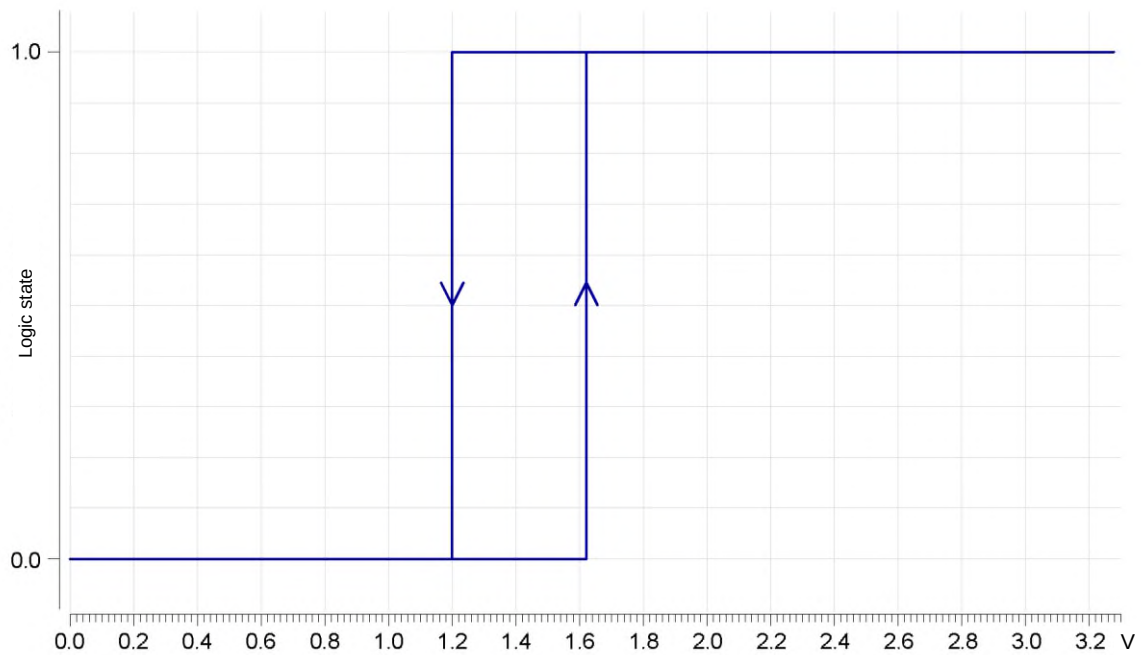
Figure 134 – Typical dependence of logic state on digital input voltage at U_{CC} = 3.3 V under nominal conditions
