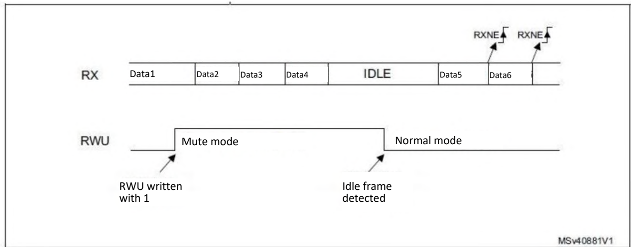
Figure 119 – Mute mode with Idle line detection
