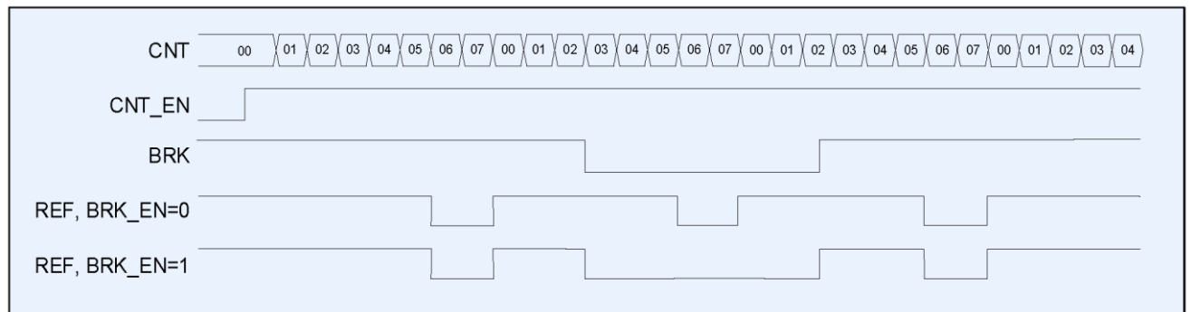
Figure 60 – REF reset timing diagram via the BRK pin
