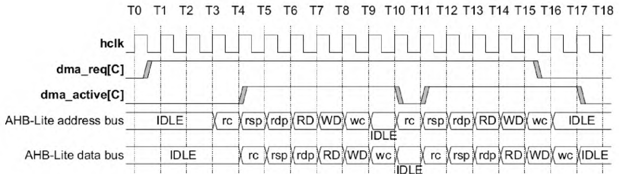
Figure 95 – Timing diagram for a level-triggered request from a peripheral block
