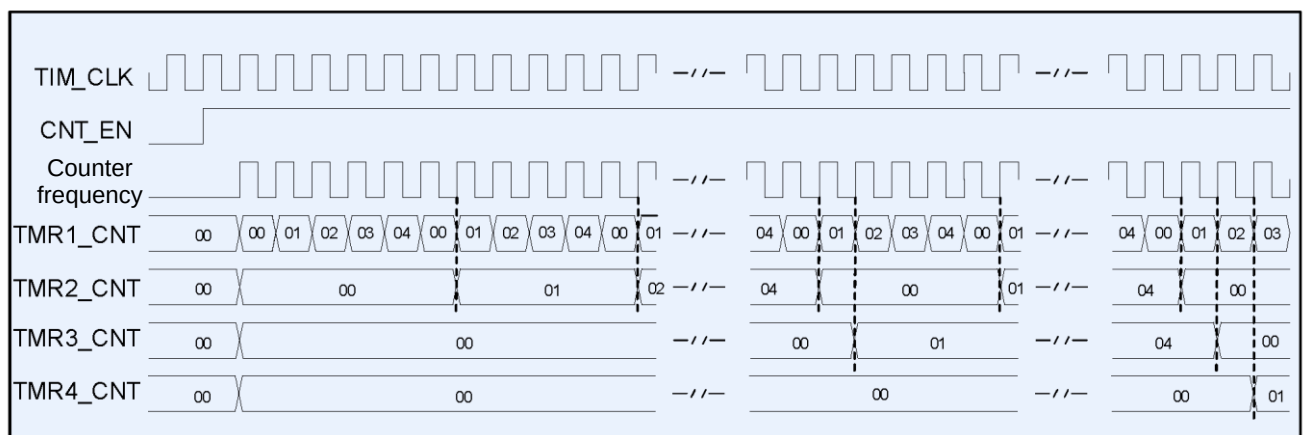
Figure 49 – Timing diagrams for four timers in cascade
