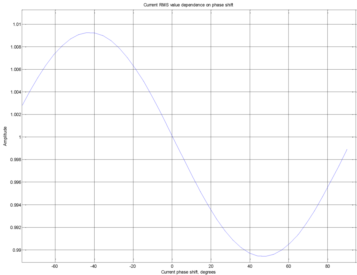
Figure 23 – Dependence of RMS on the phase shift of the input signal
