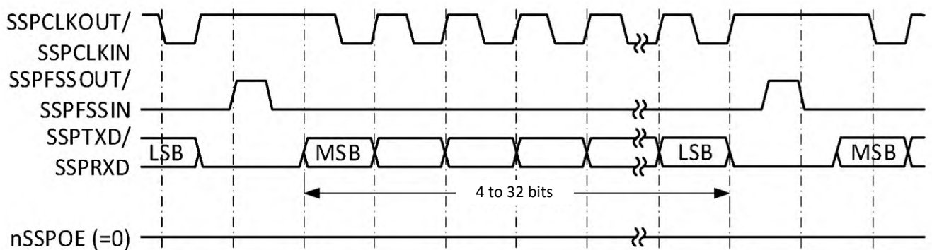
Figure 76 – SPI protocol synchronous transfer format, SPO=1, SPH = 0 (continuous transfer)
