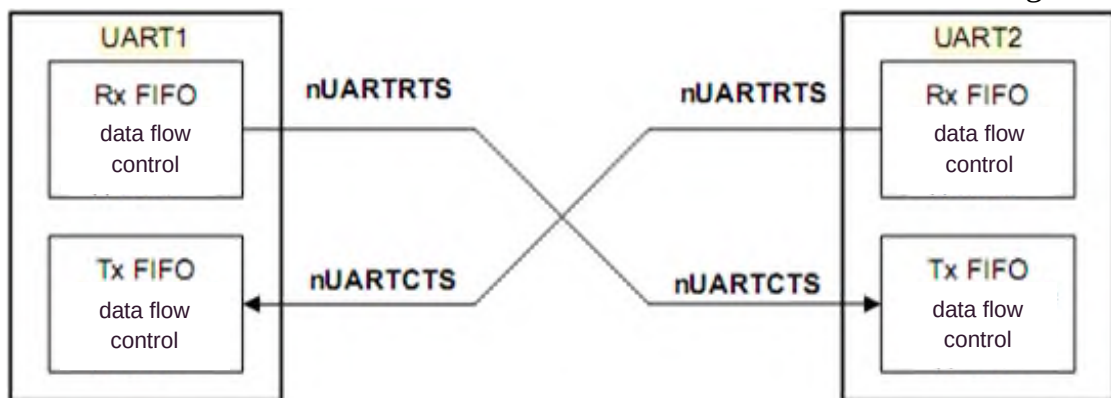
Figure 90 – Interaction between two serial devices with hardware flow control
