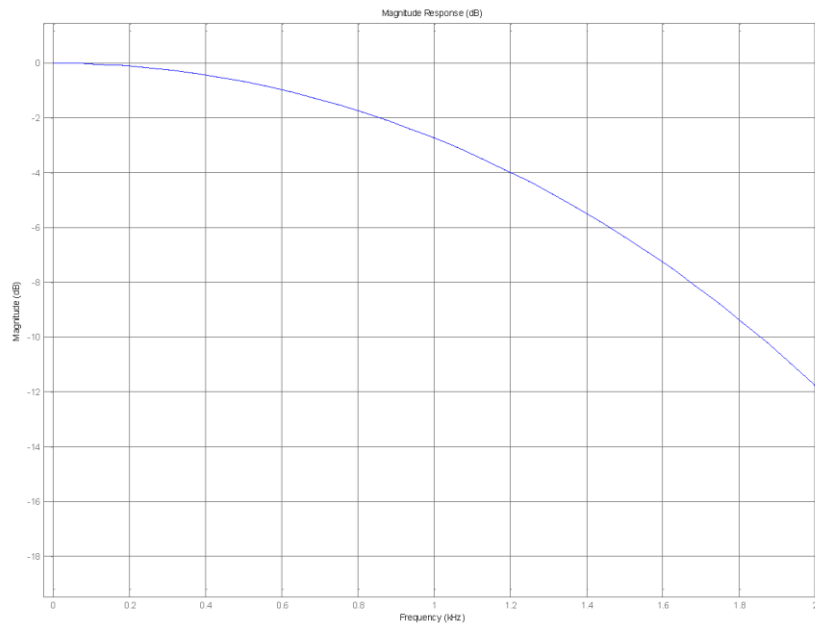
Figure 27 – Decimation filter response in the 2 kHz band
