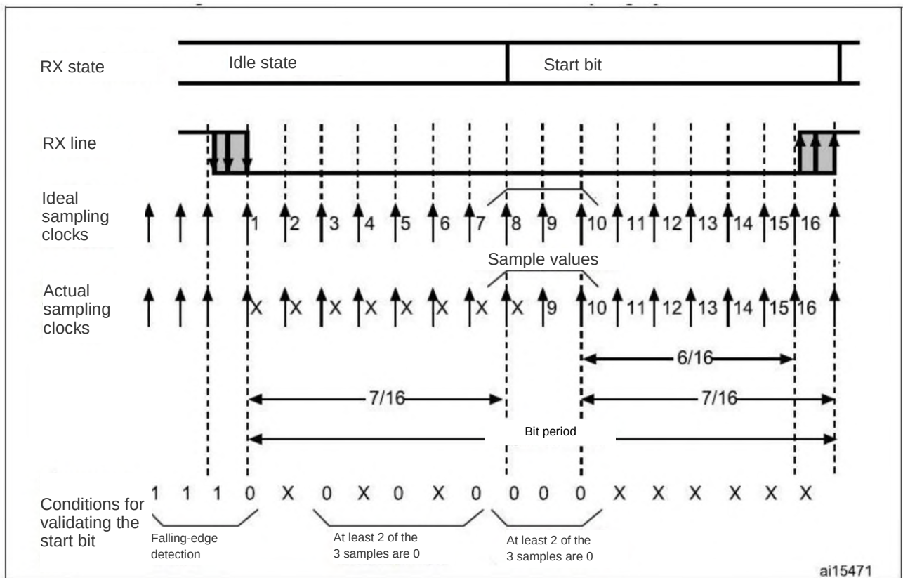
Figure 116 – Start-bit detection with oversampling by 16 and 8
