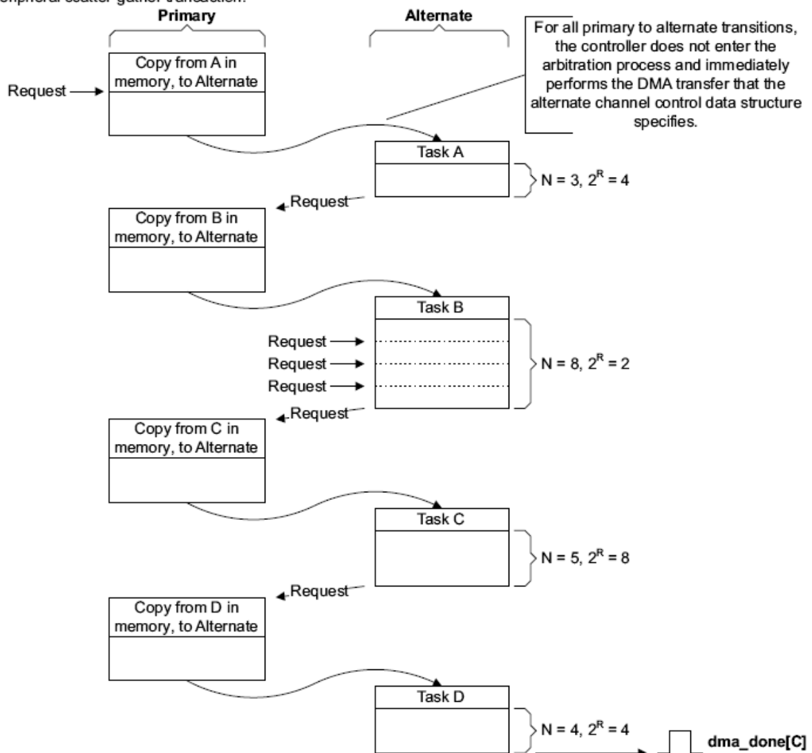
Figure 102 – Example of DMA operation in “Execution with configuration change” mode
