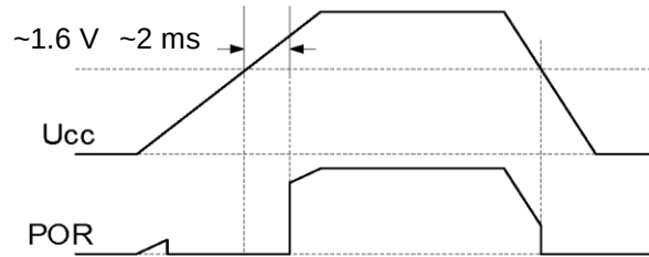
Figure 7 – Reset signal generation diagram of the integrated circuit
