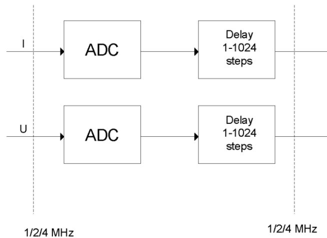
Figure 26 – Controlled phase shift in current and voltage channels
