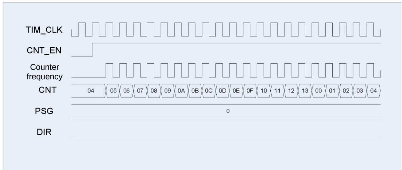
Figure 39 – Timer operation diagrams, up-counting from 0 to 0x13, start value 0x04
