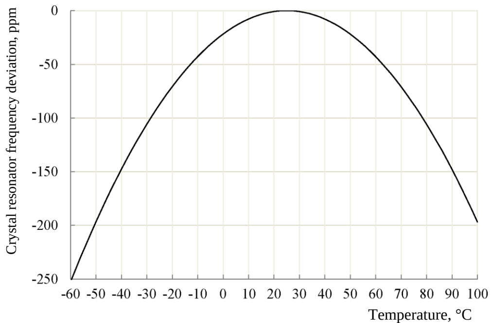
Figure 36 – Typical dependence of the frequency deviation of a 32 kHz crystal resonator on temperature
