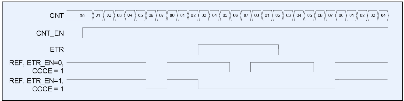
Figure 59 – REF reset timing diagram via the ETR pin
