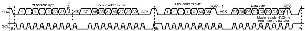
Figure 67 – I2C receive in 10-bit mode
