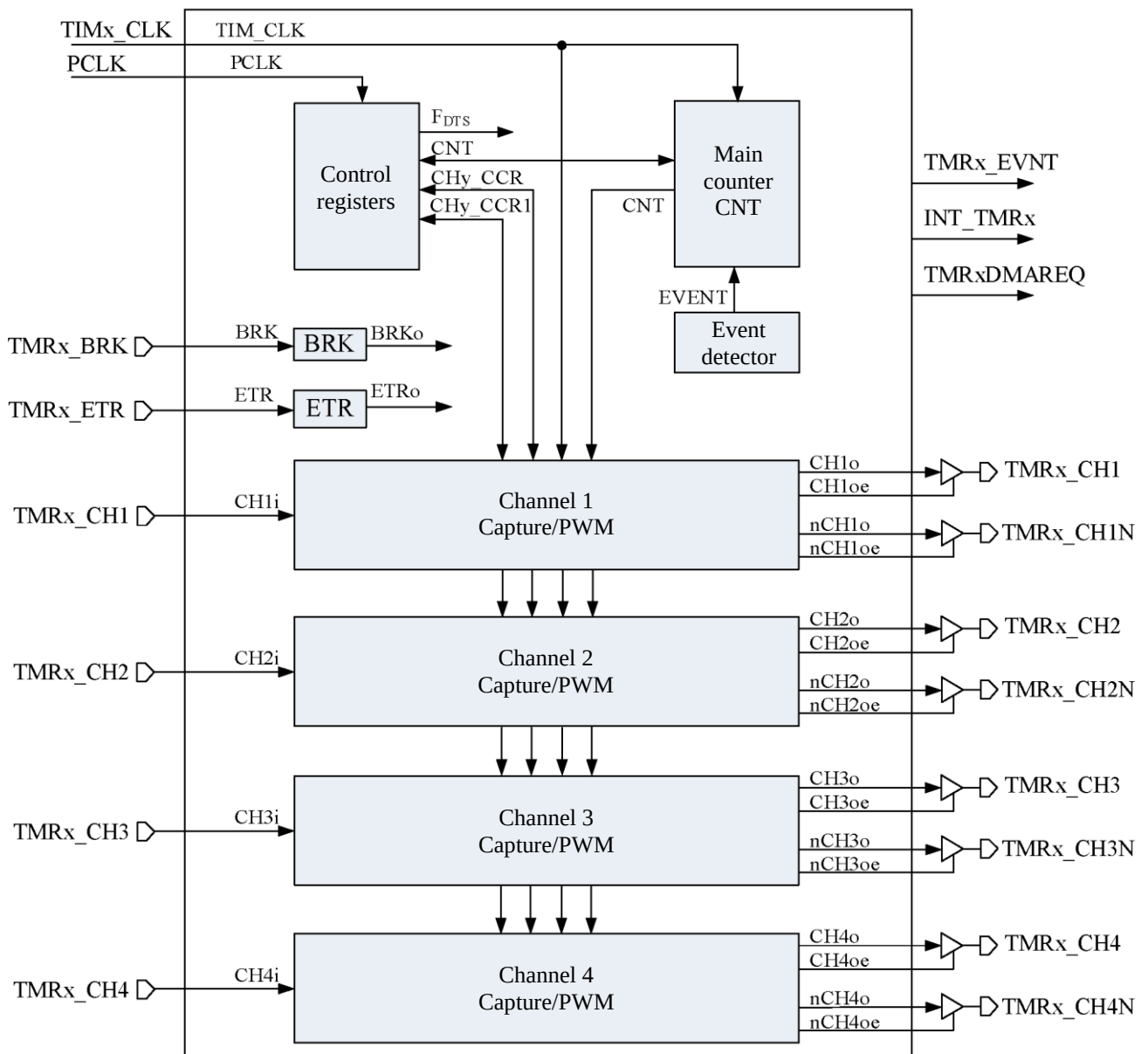
Figure 38 – Block diagram of the Timer block
