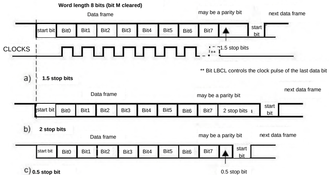
Figure 114 – Configurable stop bits
