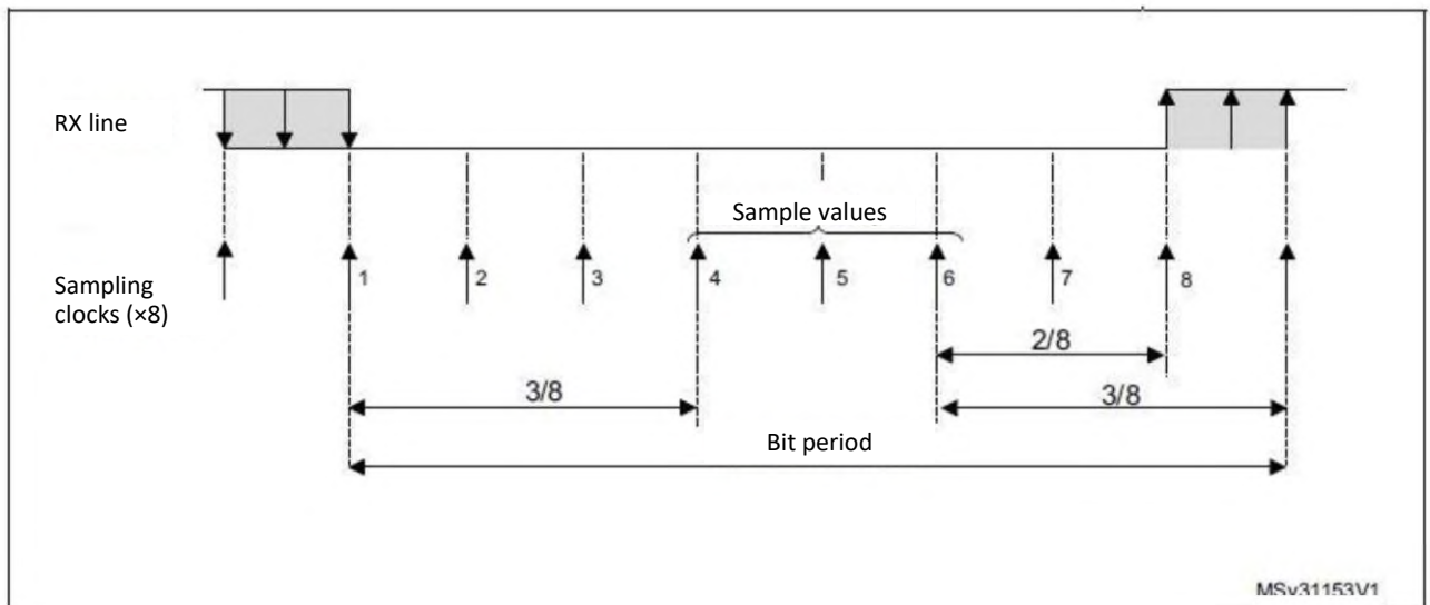
Figure 118 – Data sampling with oversampling by 8
