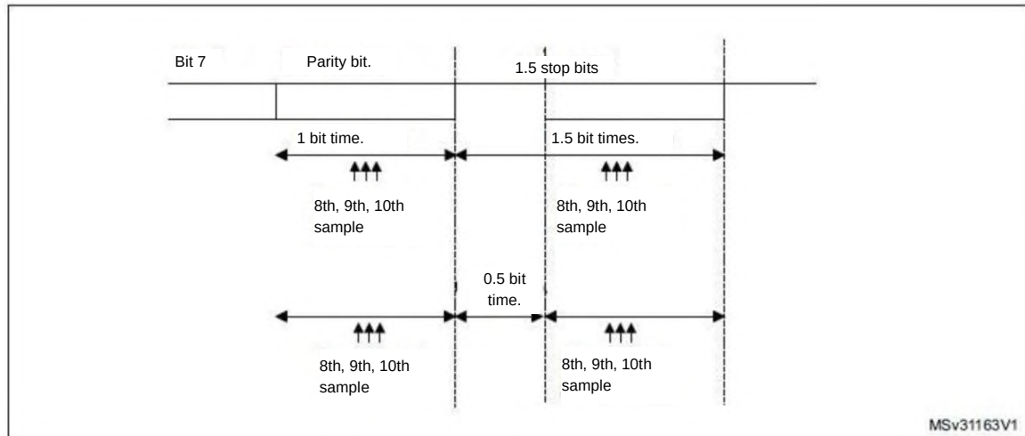
Figure 126 – Parity error detection using 1.5 stop bits
