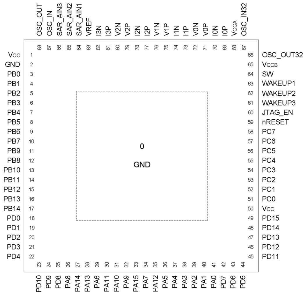
Figure 3 – Pin assignment diagram for IRL1206FI
