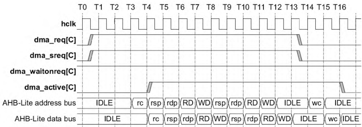
Figure 97 – DMA controller timing diagram when dma_waitonreq is used
