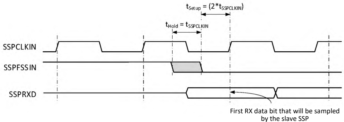
Figure 80 – Microwire format, SSPFSSIN setup and hold time requirements
