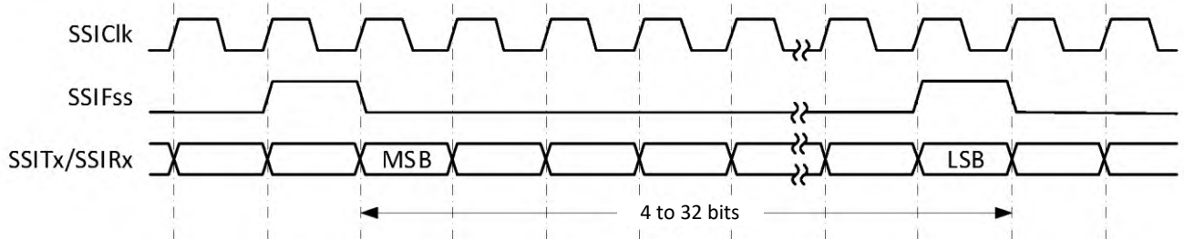
Figure 71 – SSI protocol synchronous transfer format (continuous transfer)
