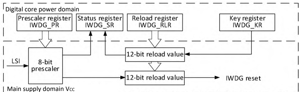
Figure 108 – Block diagram of the independent watchdog timer
