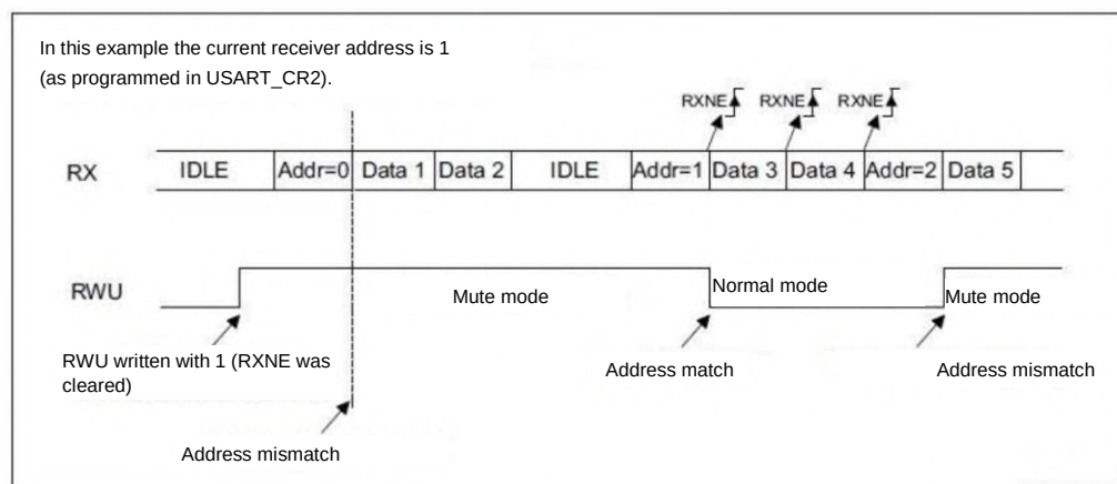
Figure 120 – Mute mode with address mark detection
