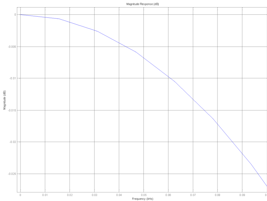
Figure 28 – Decimation filter response in the 100 Hz band
