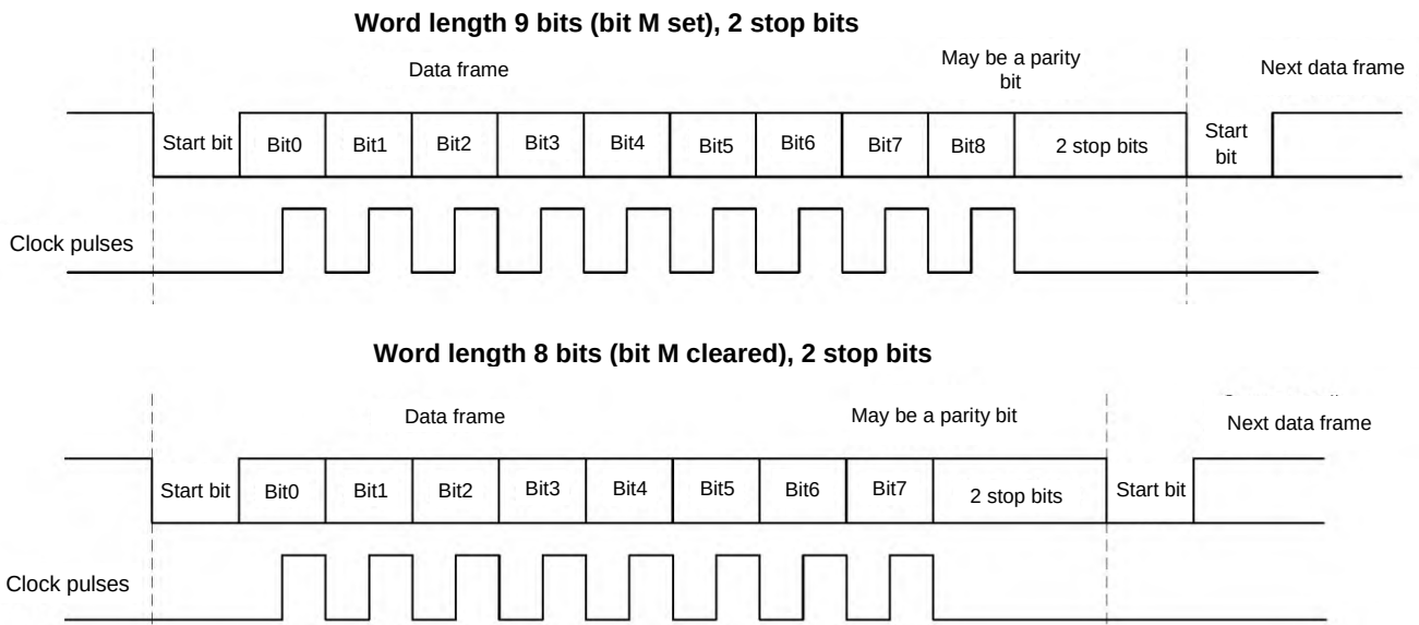
Figure 113 – Programming the word length
