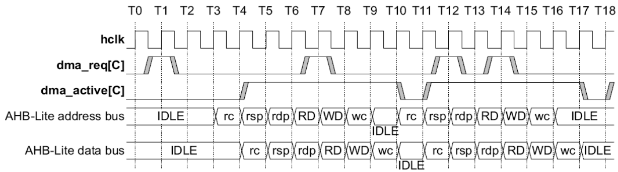
Figure 94 – Timing diagram for a pulse-triggered request from a peripheral block
