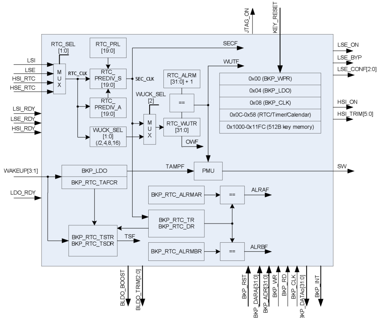
Figure 34 – Block diagram of the battery domain and the real-time clock
