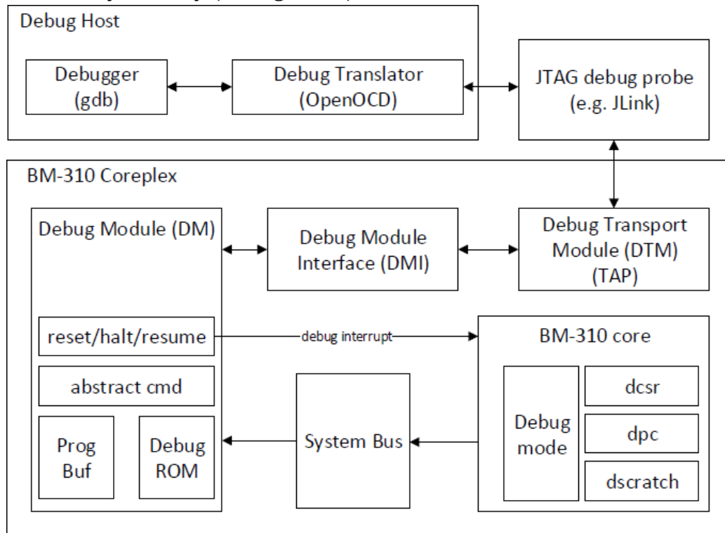
Figure 105 – Debug system architecture
