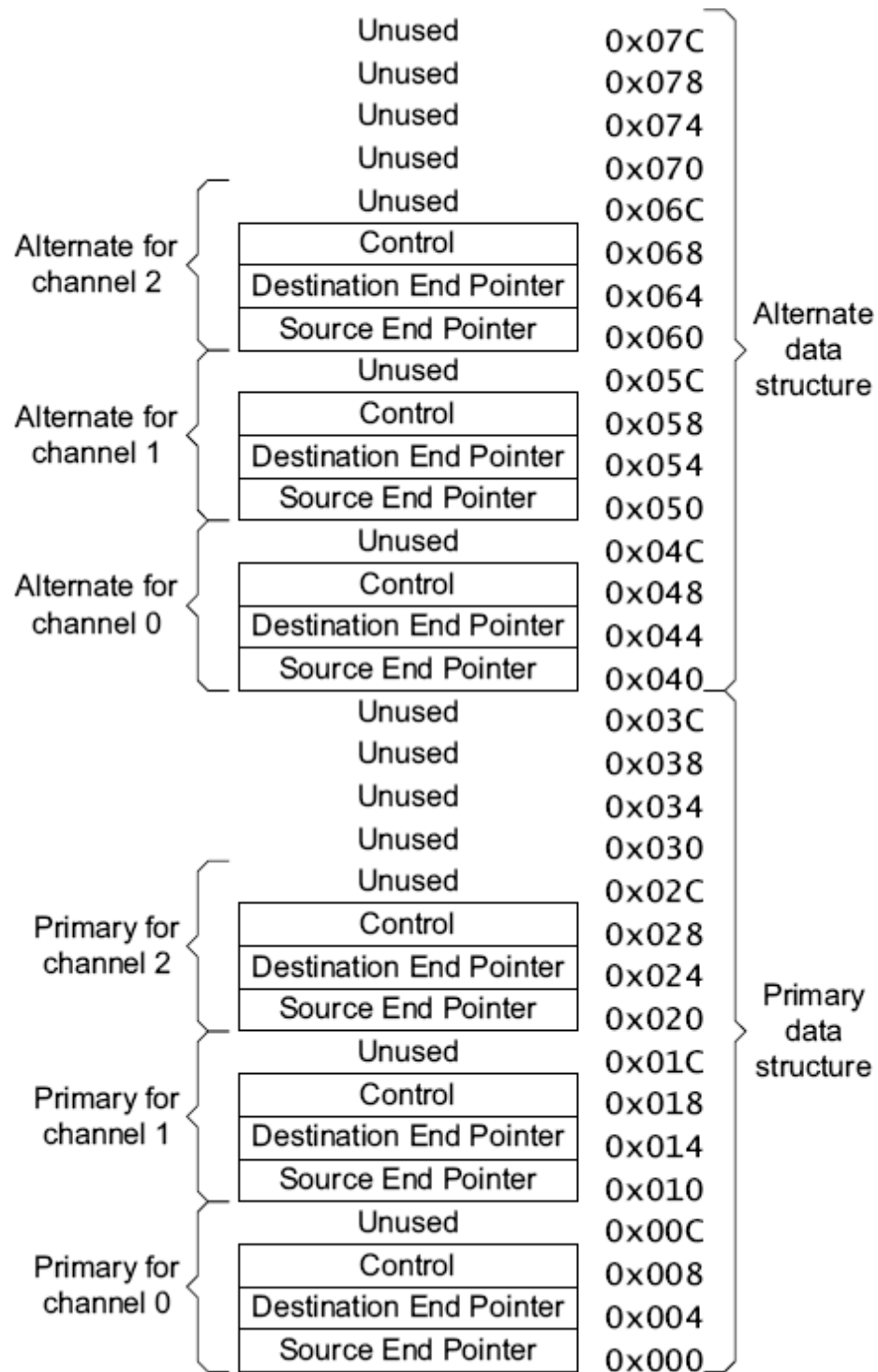
Figure 104 – Memory map for three DMA channels including an alternate control data structure (where “Destination end pointer” is the destination data end pointer; “Source end pointer” is the source data end pointer; “Control” is the control word)
