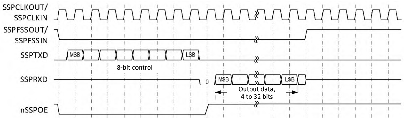
Figure 78 – Microwire protocol synchronous transfer format (single transfer)
