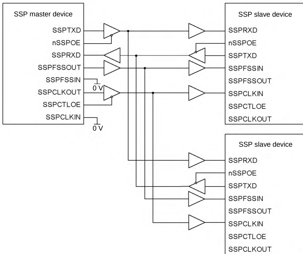
Figure 81 – SSP master device connected to two SSP slaves
