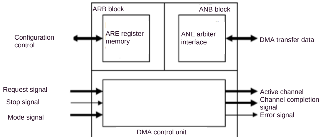
Figure 93 – Controller block diagram
