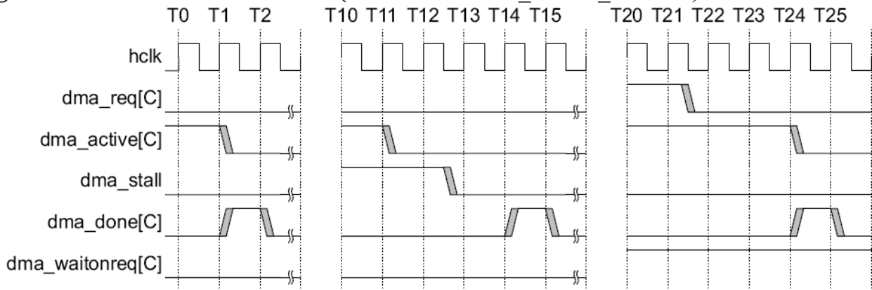
Figure 96 – dma_done operation diagrams
