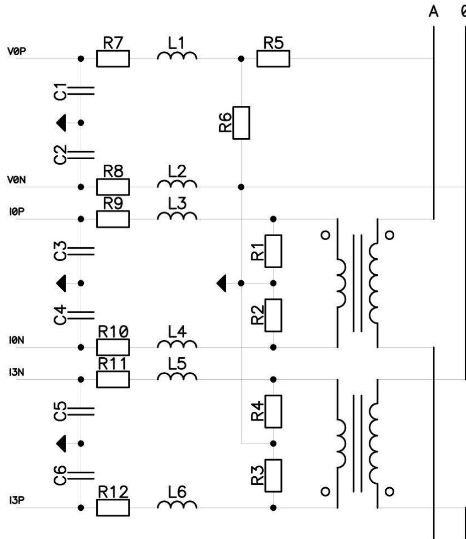
Figure 31 – Typical connection scheme for single-phase energy metering
