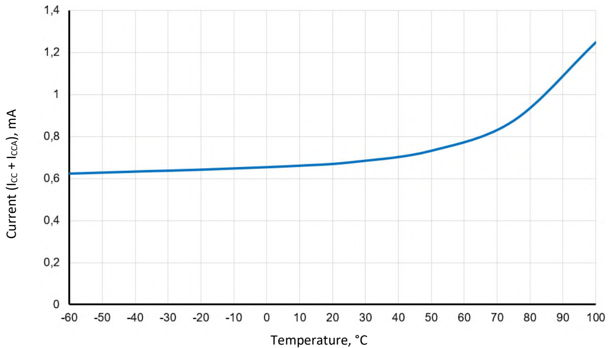
Figure 139 – Dependence of total static current (nRESET = 0) I_{CC} and I_{CCA} of IRL1206FI (CHIP_ID = 217) on temperature at U_{CC} = U_{CCA} = 3.3 V
