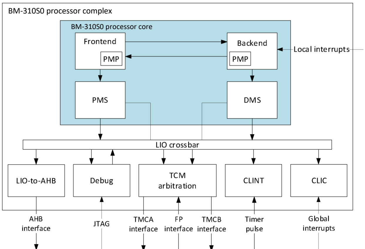
Figure 17 – Processor block diagram
