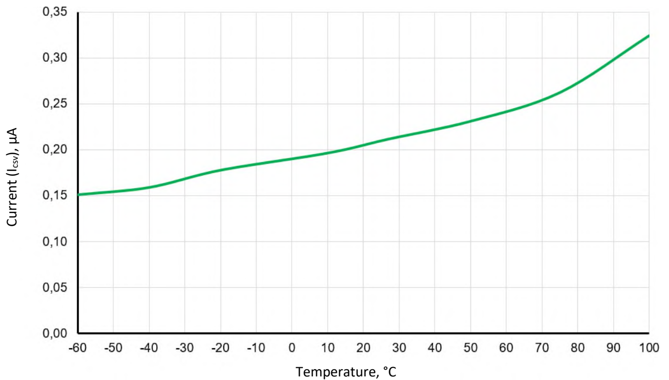
Figure 137 – Dependence of static battery-domain current I_{CCB} of IRL1206FI (CHIP_ID = 217) on temperature at U_{CCB} = 3.3 V
