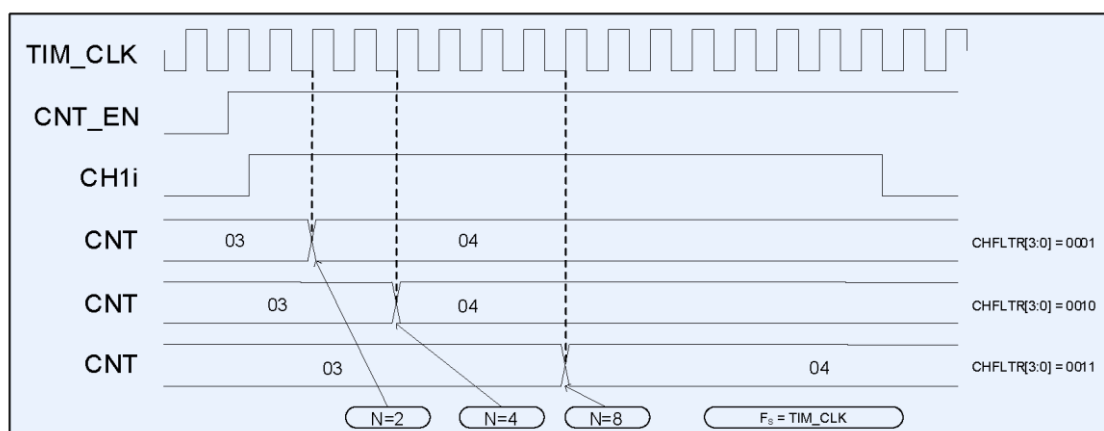
Figure 51 – External clocking timing diagram for different filter options
