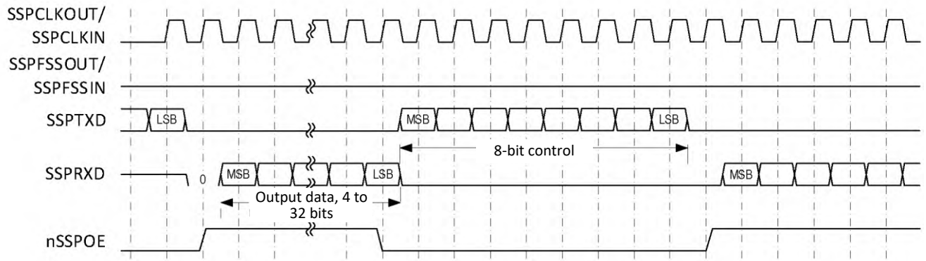
Figure 79 – Microwire protocol synchronous transfer format (continuous transfer)
