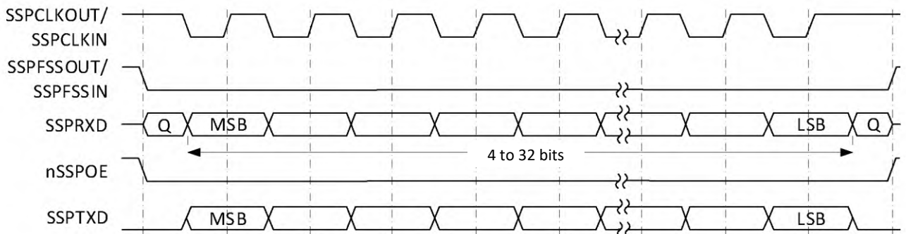
Figure 77 – SPI protocol synchronous transfer format, SPO=1, SPH=1
