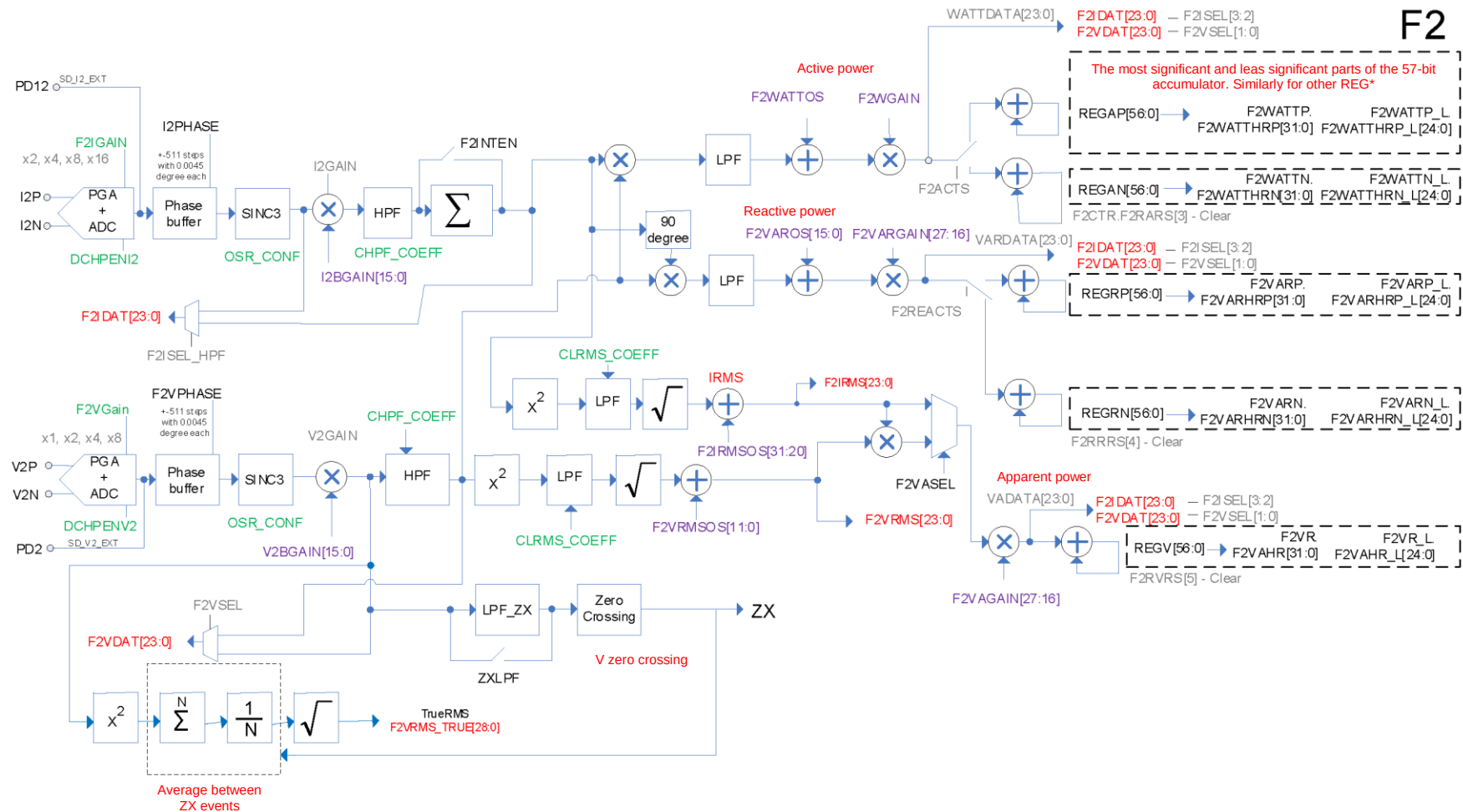
Figure 22 – Block diagram of F2
