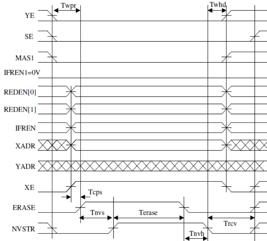
Figure 14 – Memory page erase timing diagram
