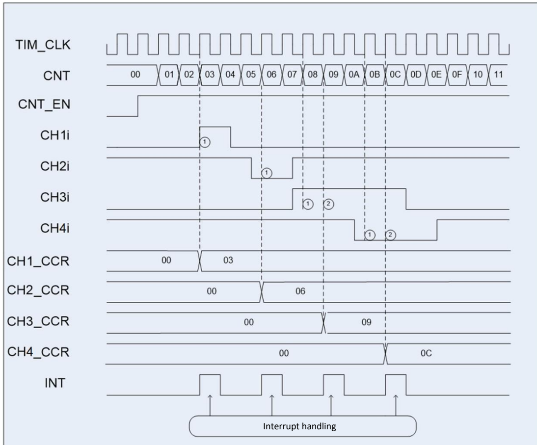
Figure 65 – Example timing diagrams in capture mode
