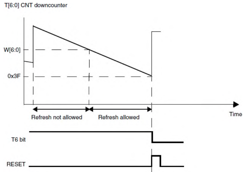
Figure 110 – Timing diagram of the window watchdog timer
