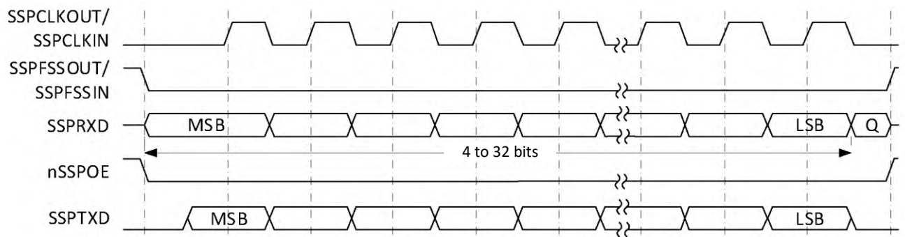
Figure 72 – SPI protocol synchronous transfer format, SPO = 0, SPH = 0 (single transfer)
