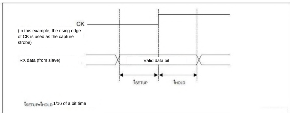
Figure 124 – RX setup/hold time
