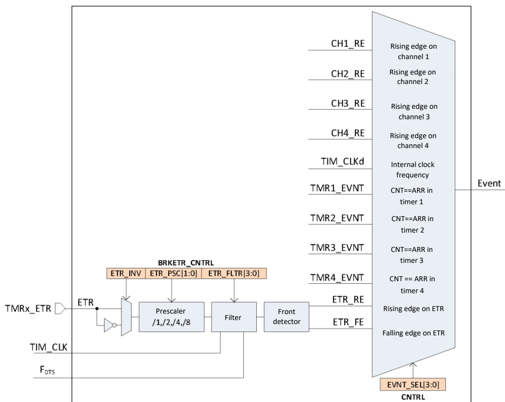
Figure 52 – Clocking scheme from the ETR input
