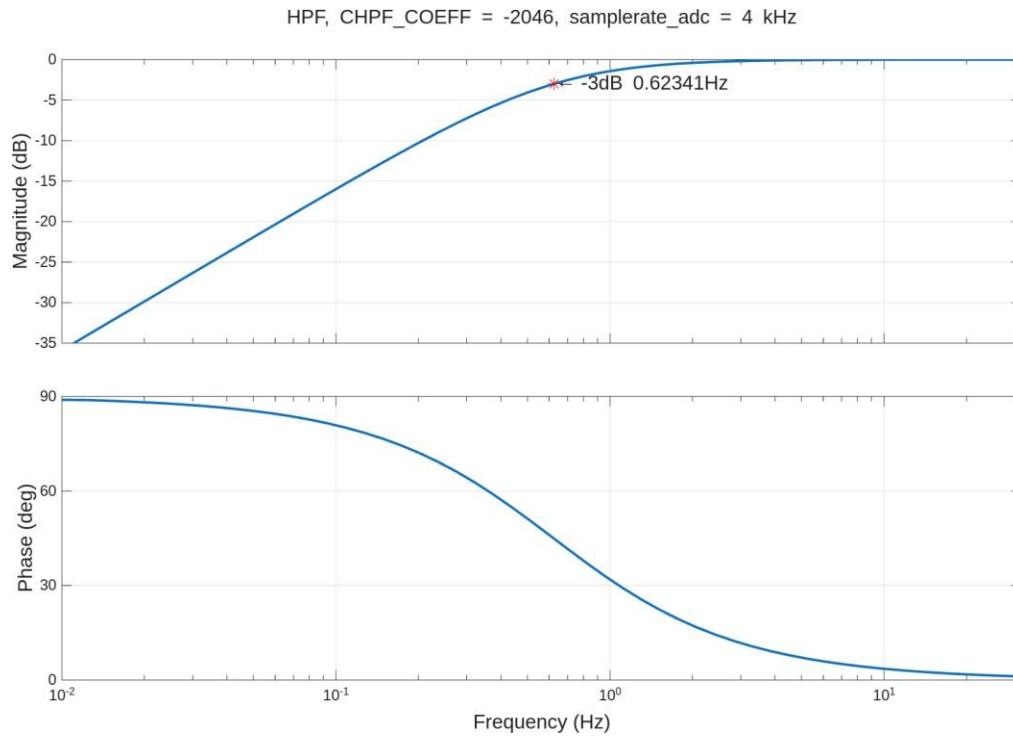
Figure 18 – Amplitude and phase frequency responses of the HPF filter with default settings at 4 kHz
