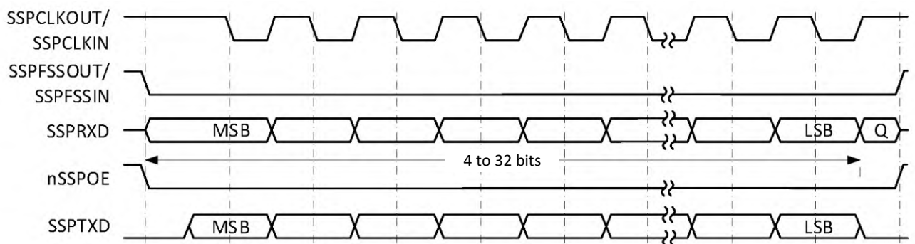
Figure 75 – SPI protocol synchronous transfer format, SPO=1, SPH=0 (single transfer)
