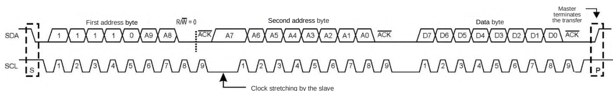
Figure 68 – I2C transmit in 10-bit mode
